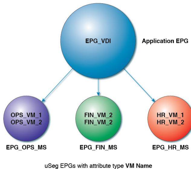
Figure 1: Microsegmentation with Cisco ACI with VMs from a Single Application EPG
