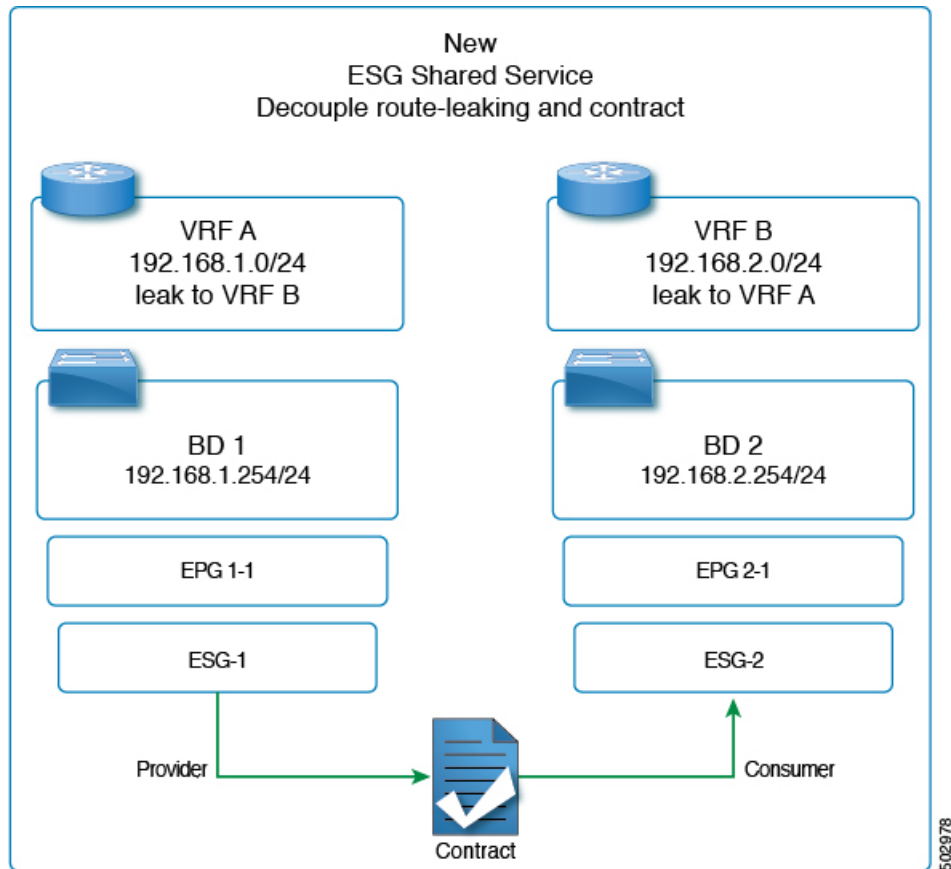
Figure 7: Route Leaking with ESGs
