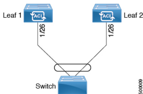
Figure 26: Switch Virtual Port Channel Configuration
