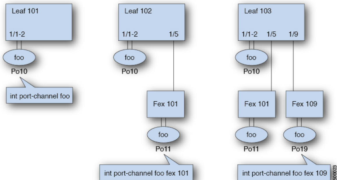
Figure 21: Example with port channels on leaf switches and FEX ports
