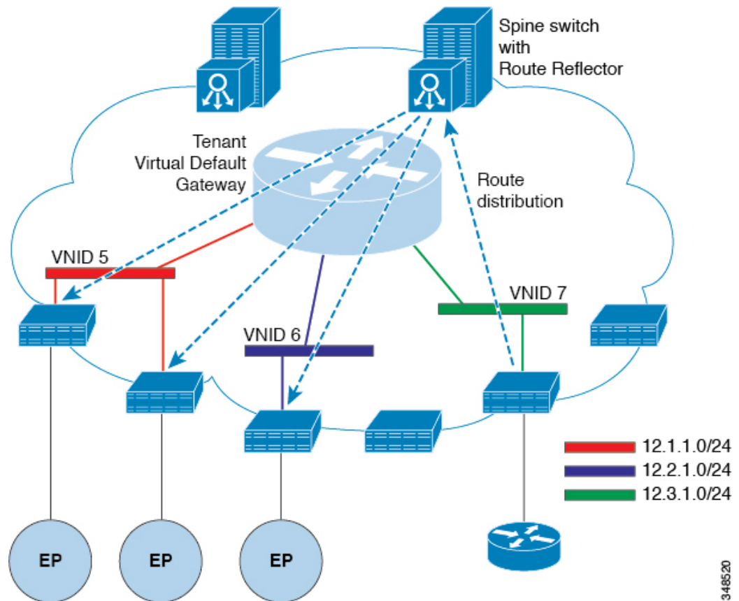
Figure 9: Router Peering
