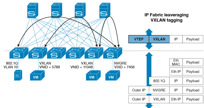
Figure 42: ACI Encapsulation Normalization
