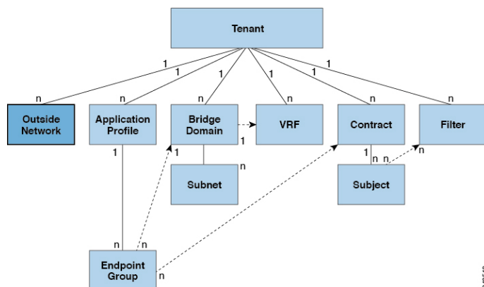
Figure 19: Outside Networks
