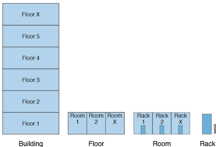
Figure 40: Geolocation
