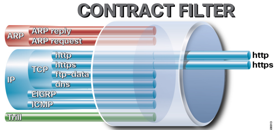
Figure 48: Contract Filters
