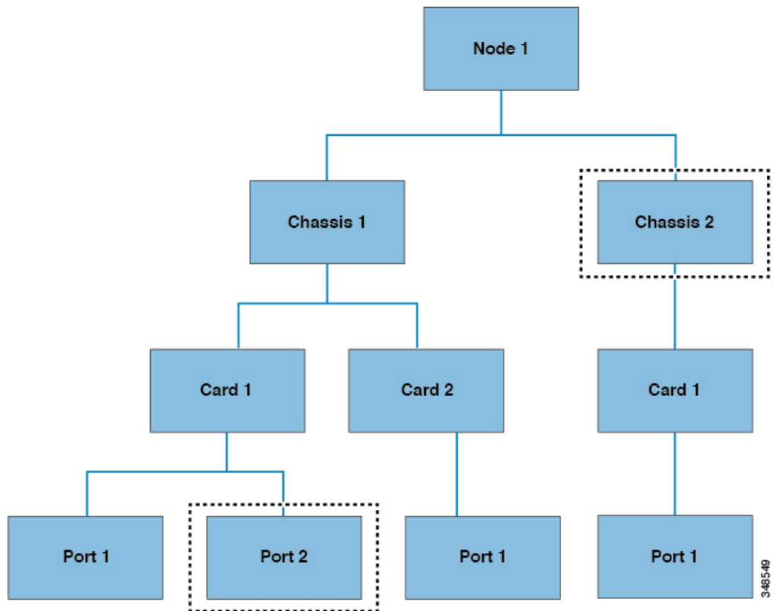
Figure 122: Object-Level Queries
