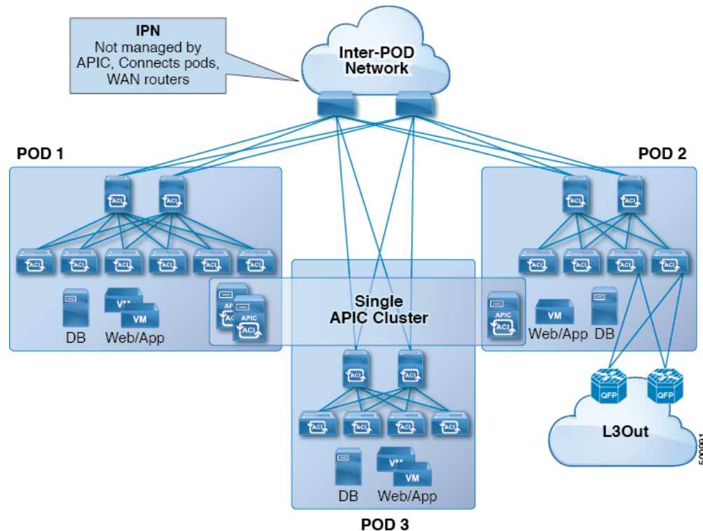
Figure 77: Multipod Overview
