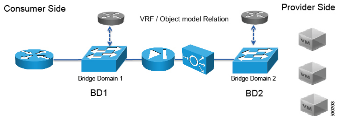
Figure 104: Bridge Domains and VRF instances of a Service Graph
