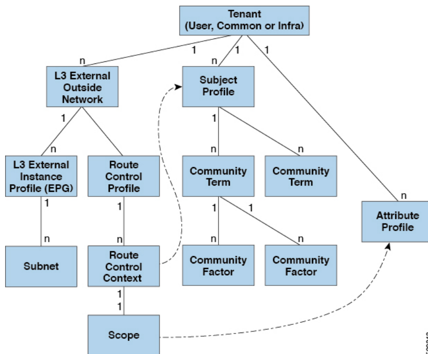
Figure 72: Route Community Matching
