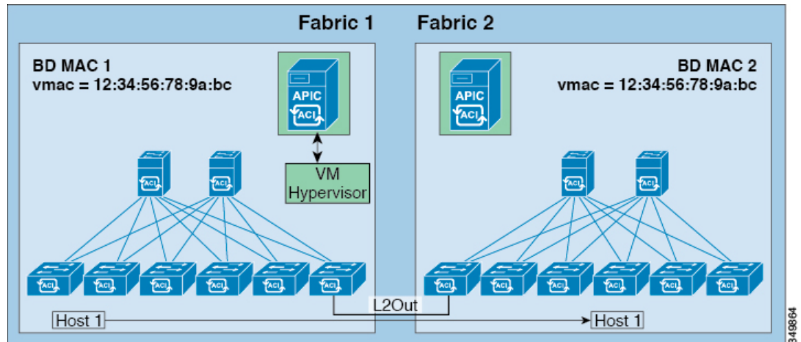
Figure 66: ACI Multi-Fabric Common Pervasive Gateway
