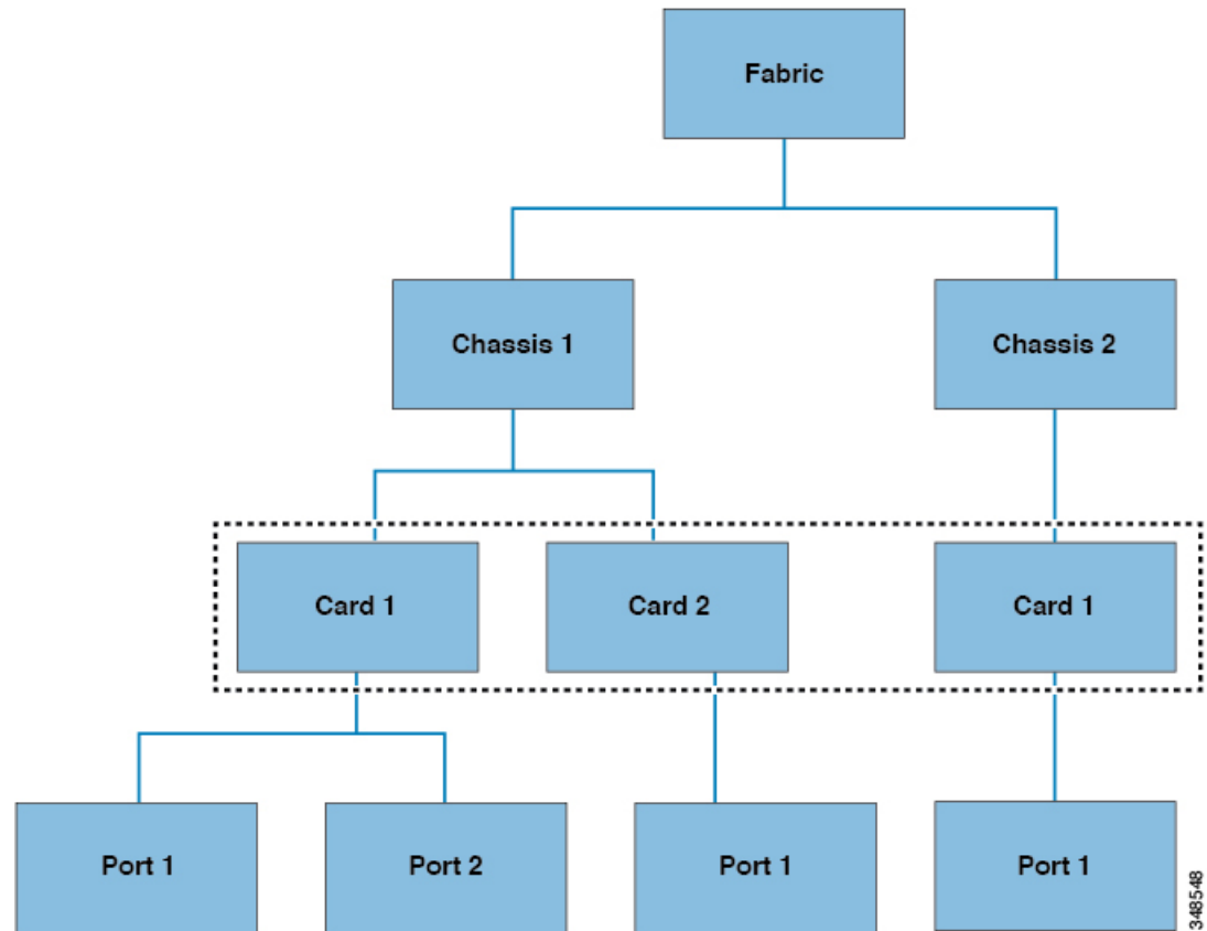
Figure 121: Class-Level Queries
