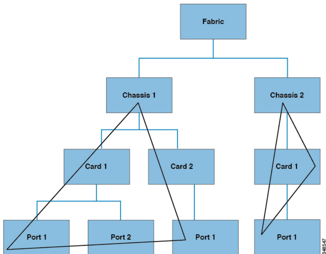
Figure 120: Tree-Level Queries
