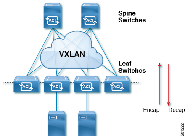
Figure 41: ACI Fabric
