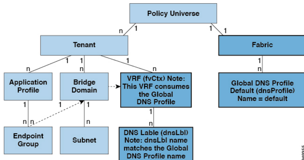
Figure 61: DNS
