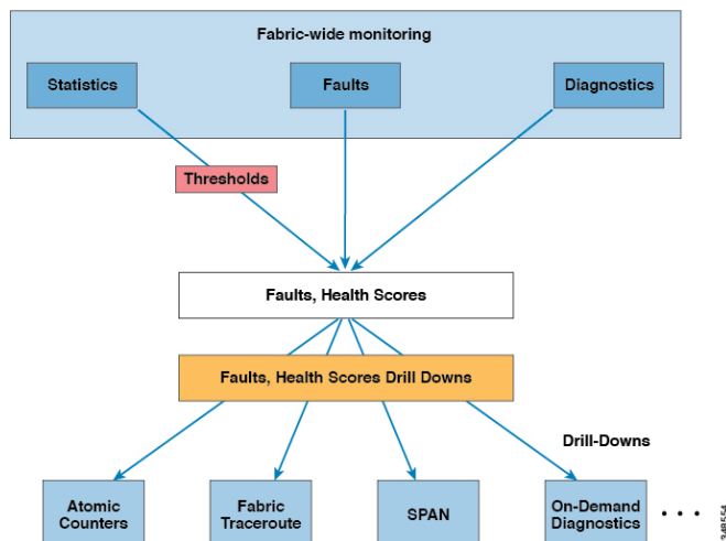
Figure 132: Troubleshooting
