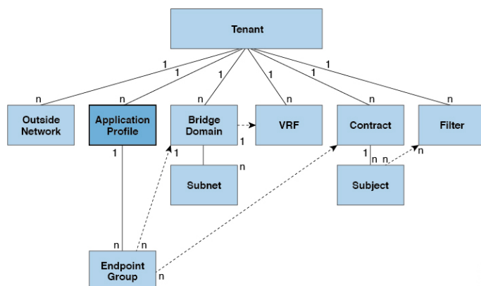
Figure 8: Application Profiles
