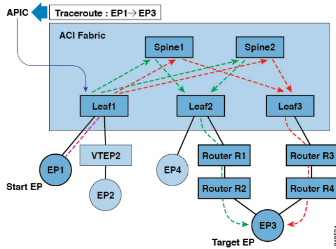
Figure 133: APIC Endpoint to Endpoint Traceroute
