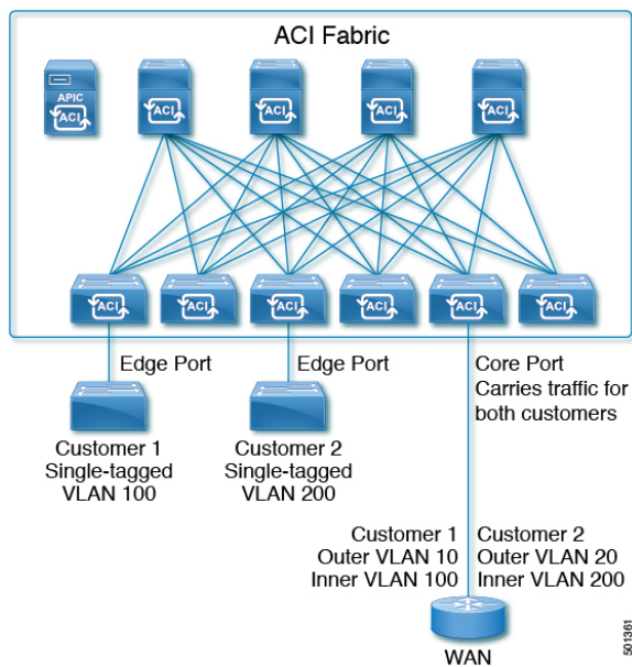
Figure 36: ACI 802.1Q Tunnels
