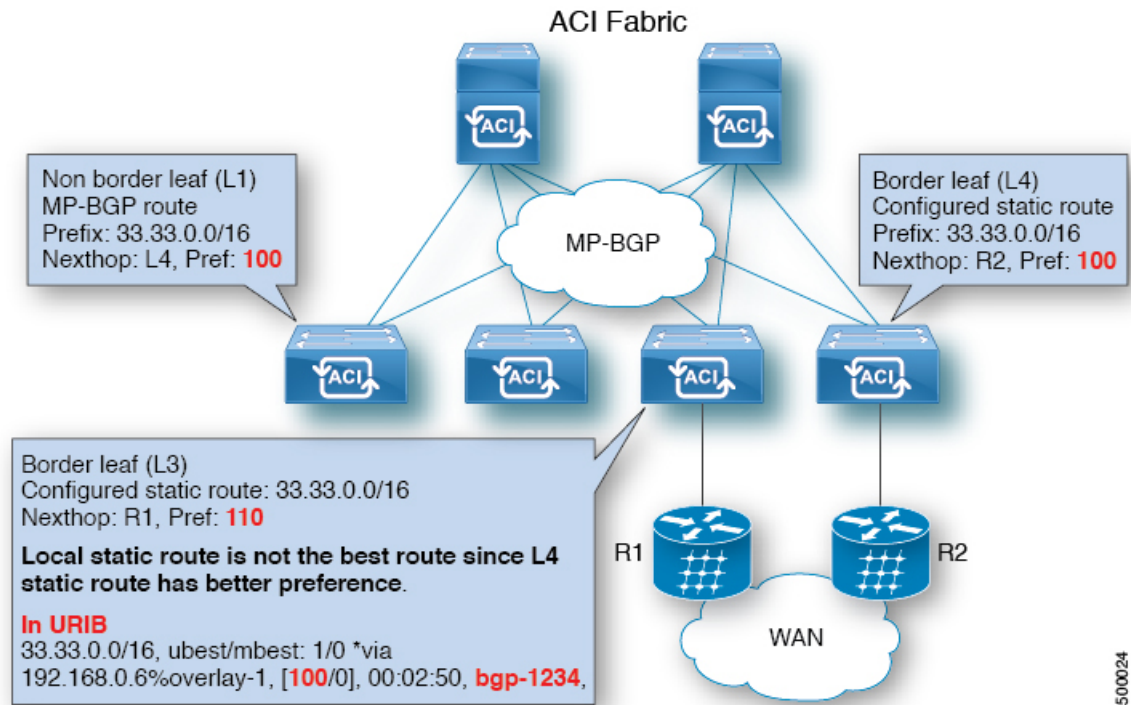
Figure 71: Static Route Preference
