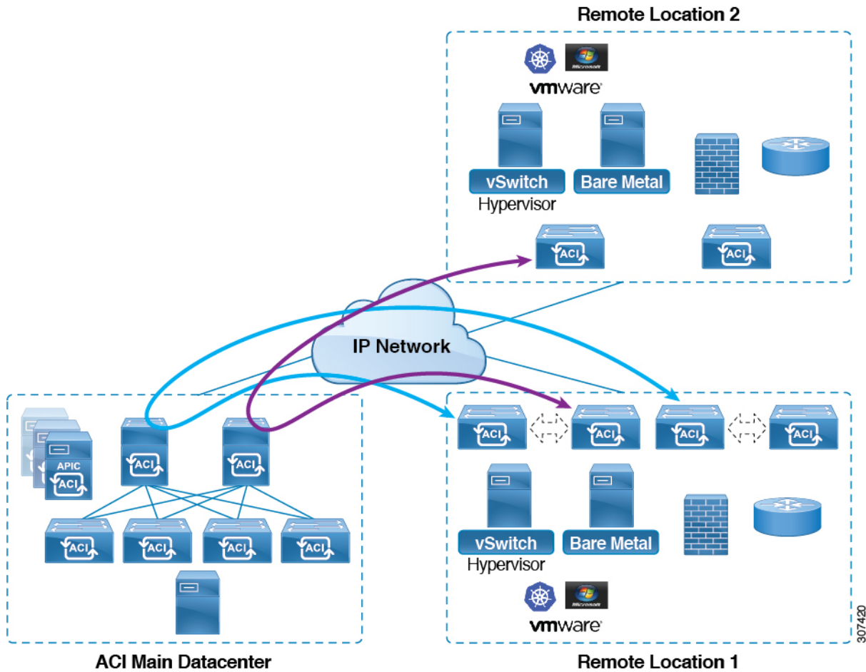
Figure 81: Remote Switching Traffic: Prior to Release 4.1(2)
