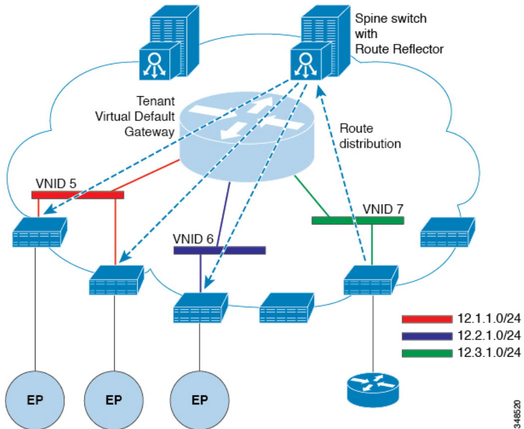
Figure 67: Router Peering
