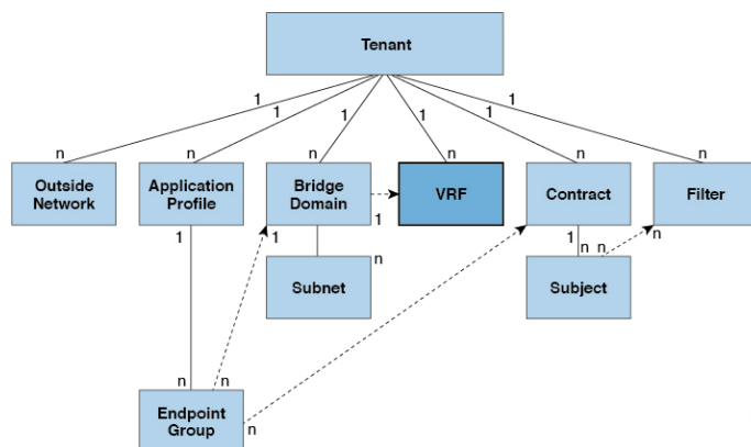
Figure 7: VRFs
