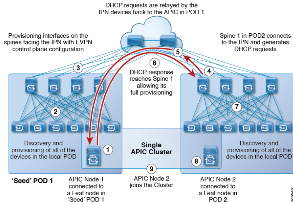
Figure 78: Multipod Provisioning
