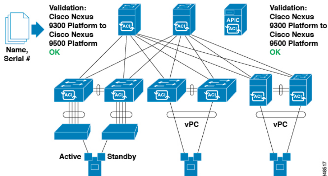
Figure 22: Fabric Provisioning
