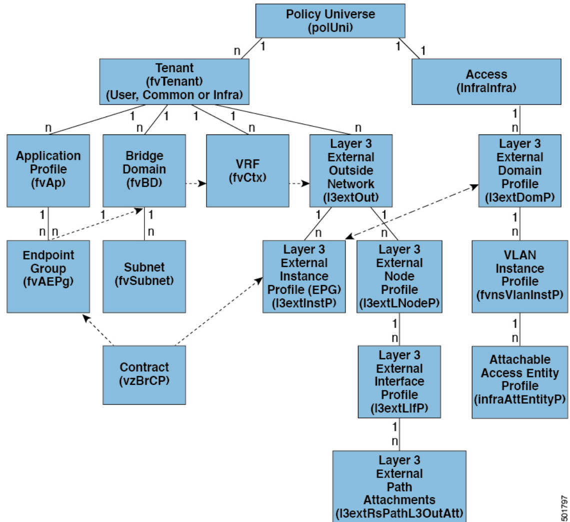
Figure 70: Policy Model for Layer 3 External Connections
