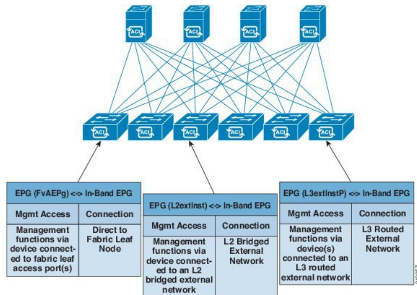
Figure 63: In-Band Management Access Scenario
