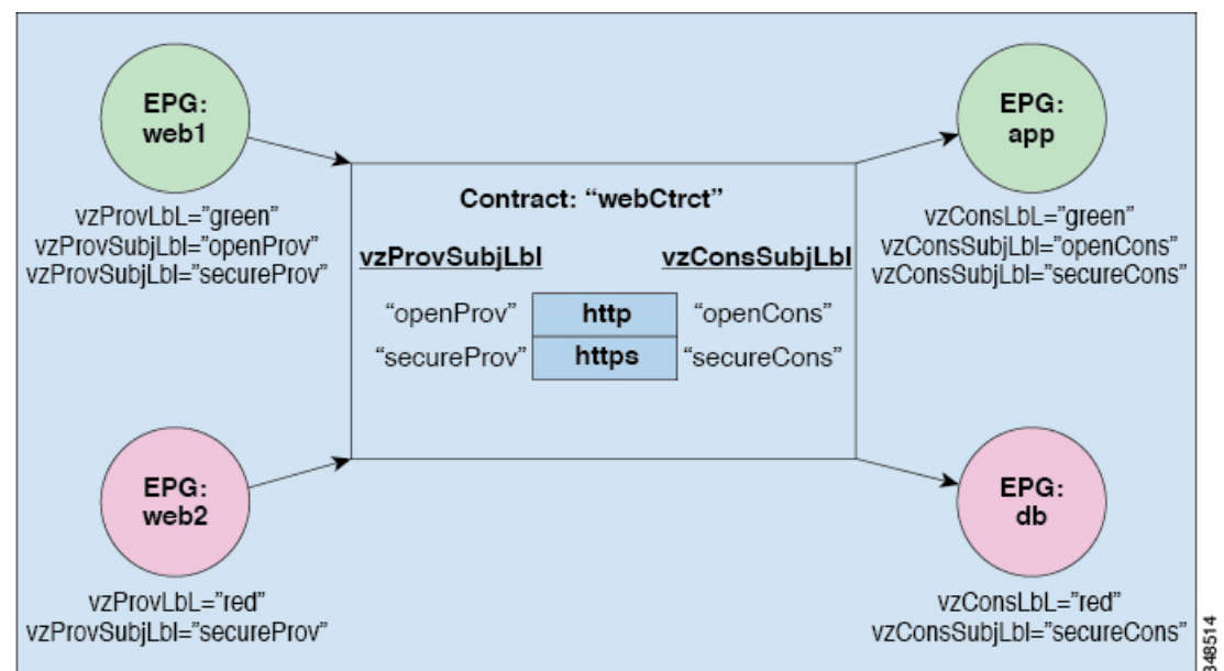
Figure 49: Contracts Determine EPG to EPG Communications
