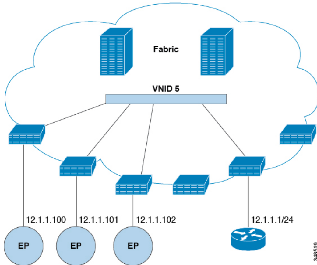
Figure 69: Bridged External Router
