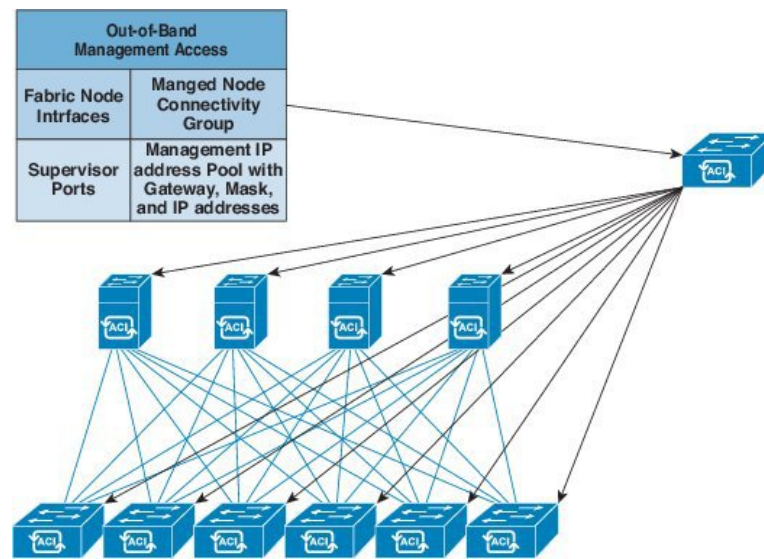
Figure 65: Out-of-Band Access Scenario
