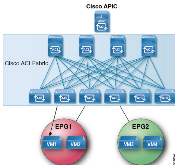
Figure 58: ACI Fabric Sends a Proxy ARP Response to VM1
