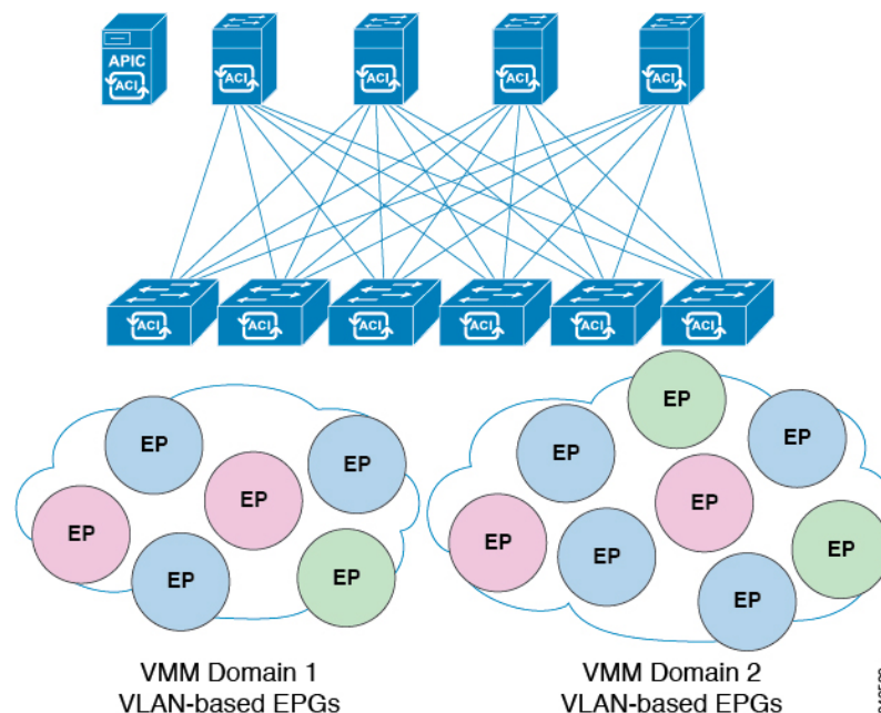
Figure 99: VMM Domain EPG Association
