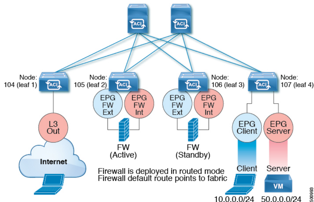
Figure 106: Sample ACI PBR Physical Topology
