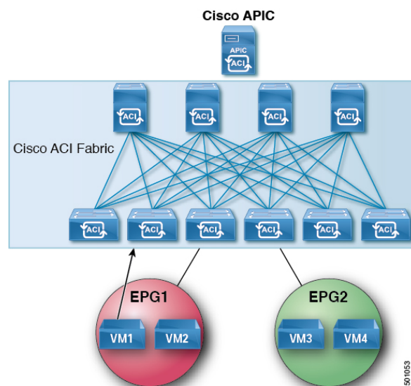
Figure 57: VM1 Sends an ARP Request with a Broadcast MAC Address to VM2
