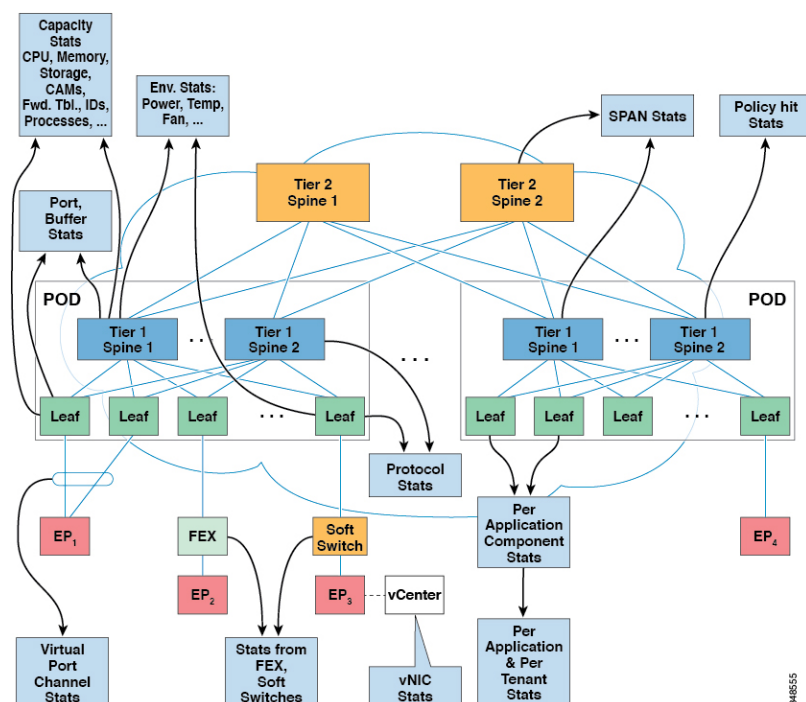
Figure 128: Various Sources of Statistics
