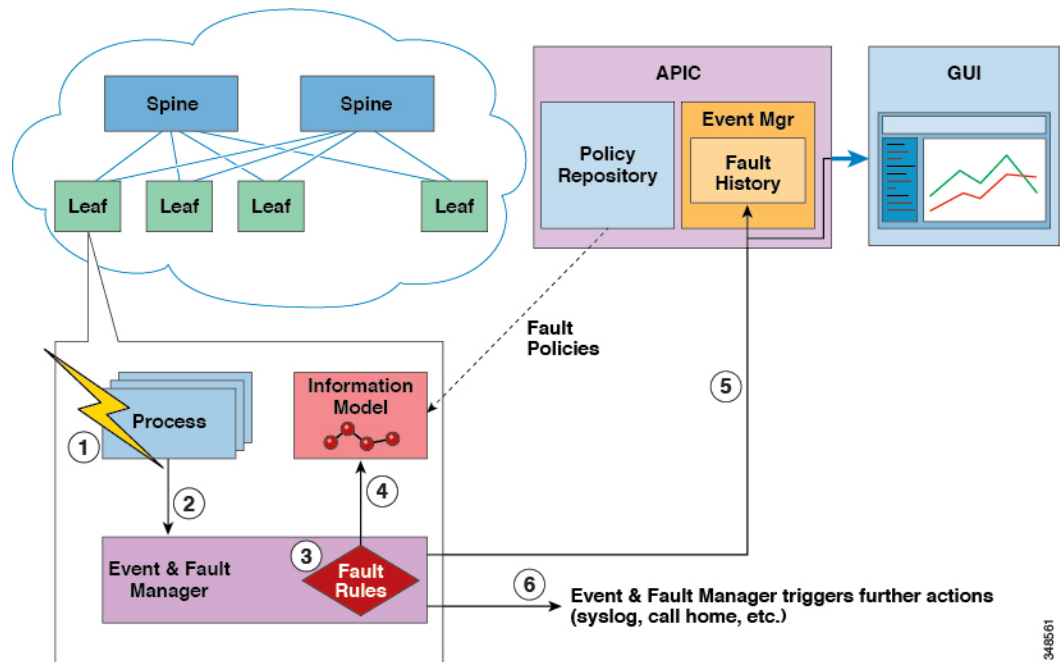
Figure 127: Faults and Events Reporting/Export
