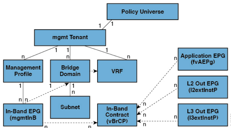
Figure 62: In-Band Management Access Policy
