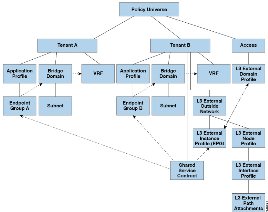
Figure 73: Shared L3Out Policy Model
