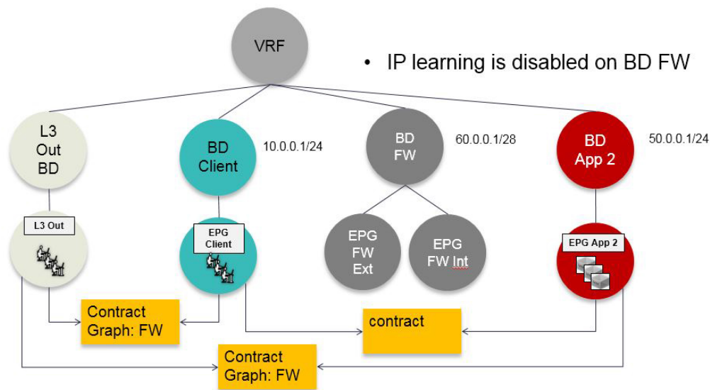
Figure 107: Sample ACI PBR Logical Topology
