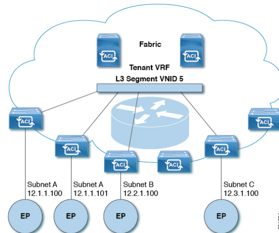
Figure 45: Layer 3 VNIDs Transport ACI Inter-subnet Tenant Traffic
