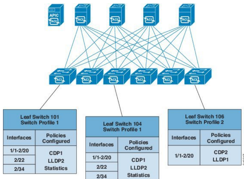
Figure 32: Applying an Access Switch Policy
