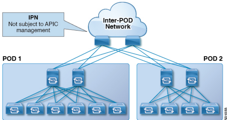
Figure 83: Multi-Pod Topology
