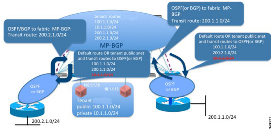
Figure 90: Route Redistribution
