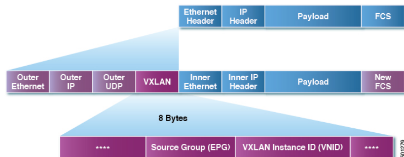
Figure 41: ACI VXLAN Packet Format
