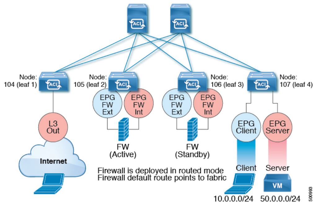
Figure 104: Sample ACI PBR Physical Topology
