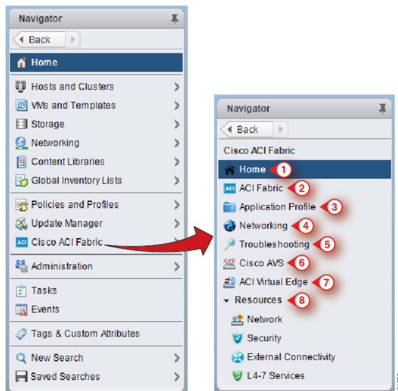
Figure 1: Main Menu
