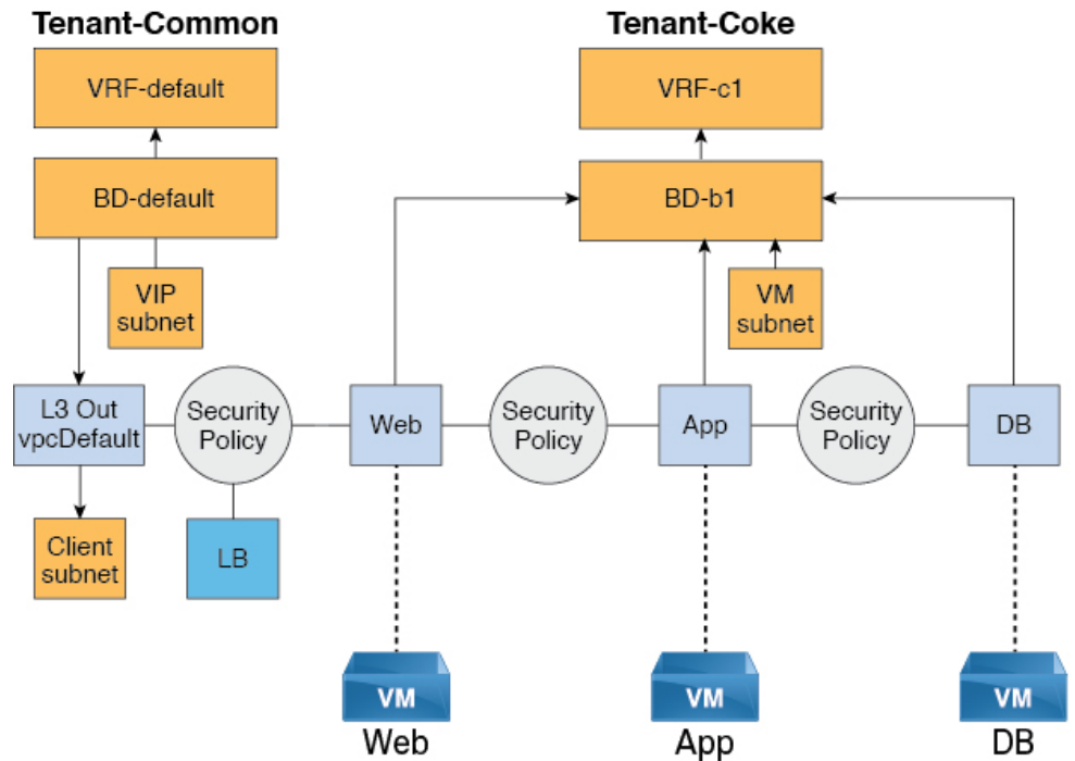
Figure 5: VPC Plan - Load Balancer Only
