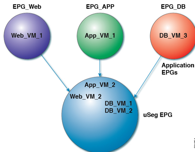
Figure 2: Microsegmentation with Cisco ACI in Different Application EPGs
