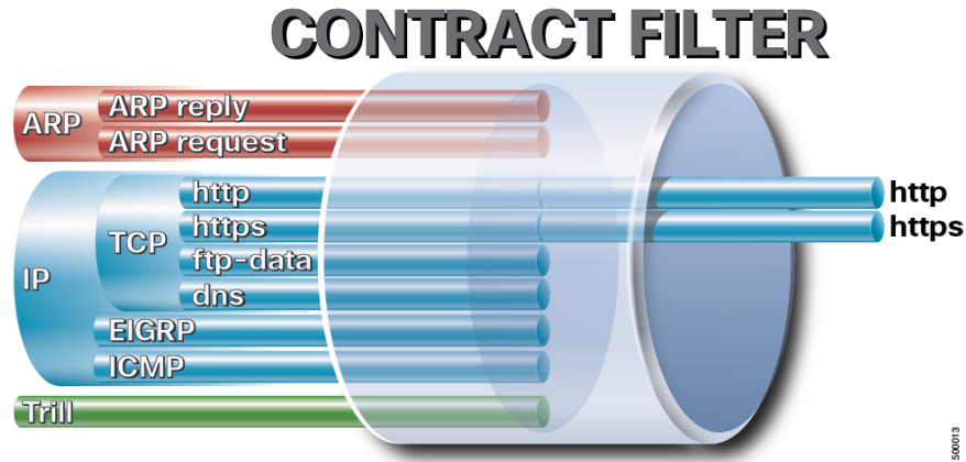
Figure 15: Contract Filters
