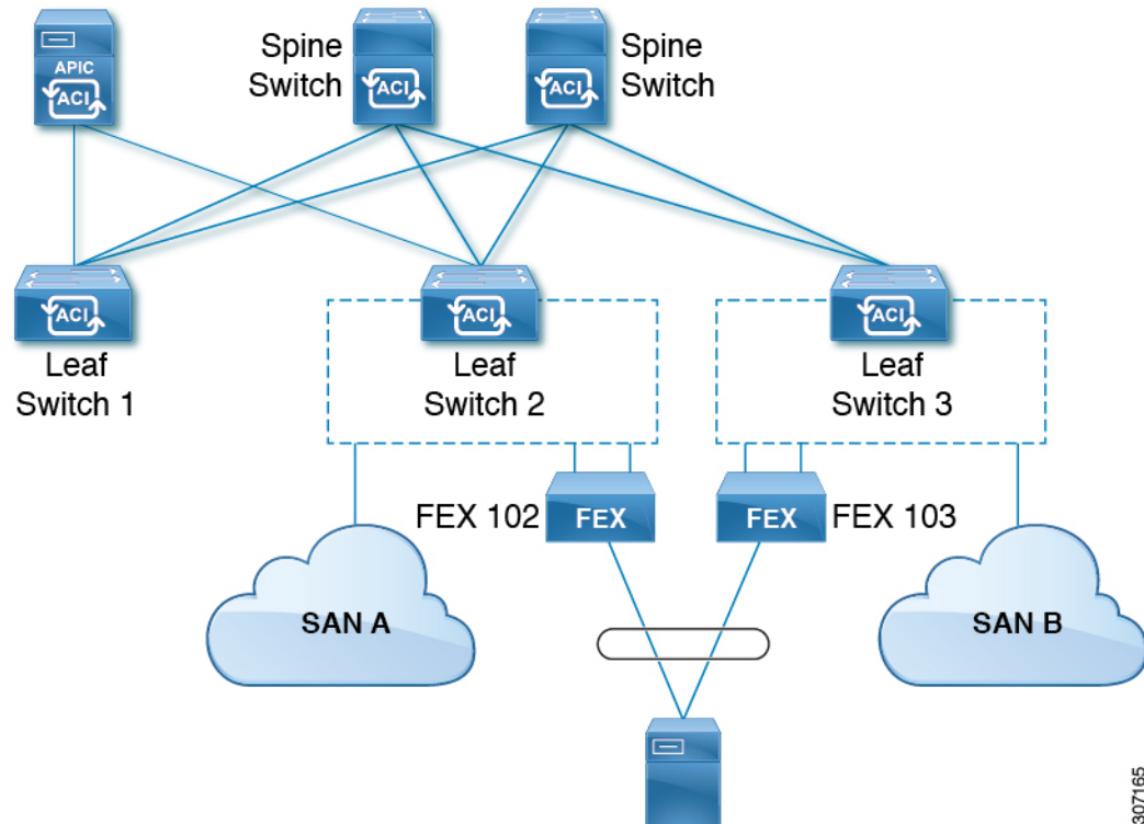
Figure 3: SAN Boot Topology with a FEX host interface (HIF) port vPC
