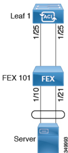
Figure 28: FEX port channel
