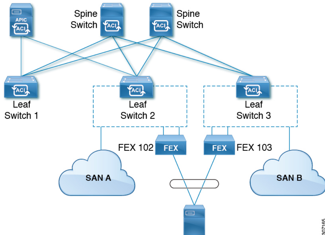
Figure 32: SAN Boot Topology with a FEX host interface (HIF) port vPC
