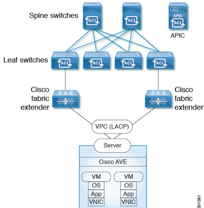
Figure 5: Cisco Fabric Extender Topology
