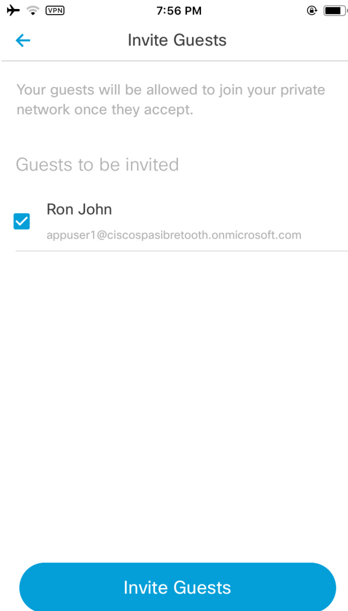
Figure 2: Invite Guest
