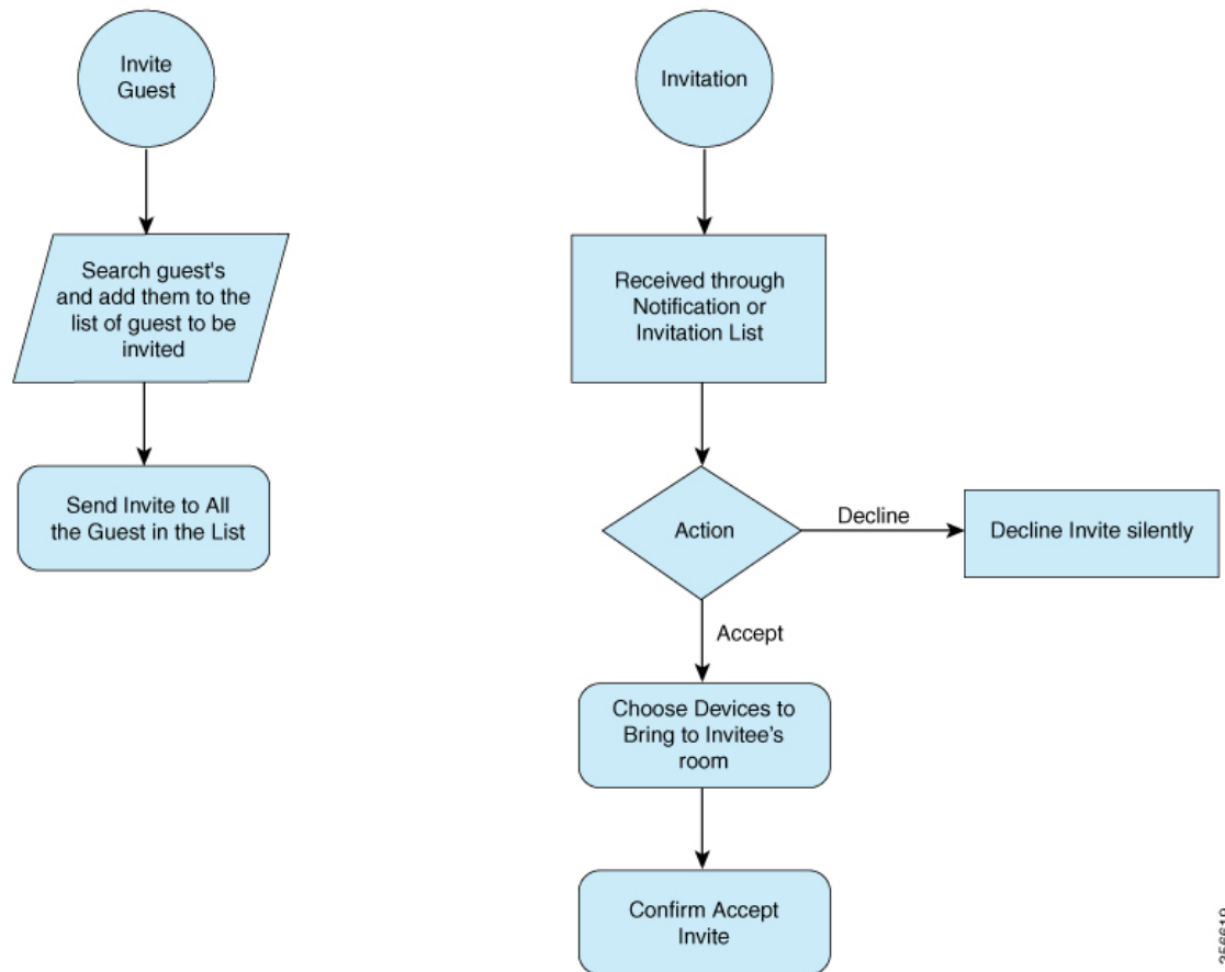
Figure 1: Invitation Flow
