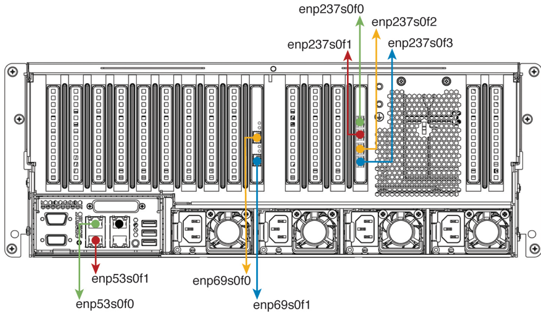
Figure 2: Recommended Cabling for 112-Core Appliance
