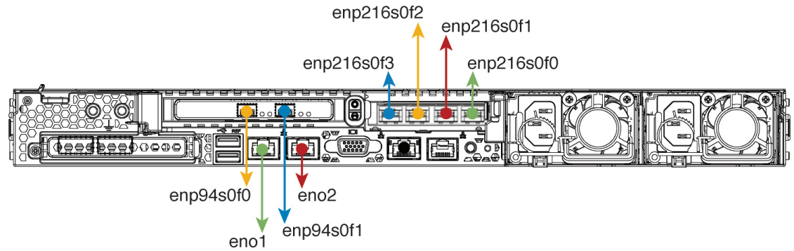
Figure 1: Recommended Cabling for 44 and 56-Core Appliance
