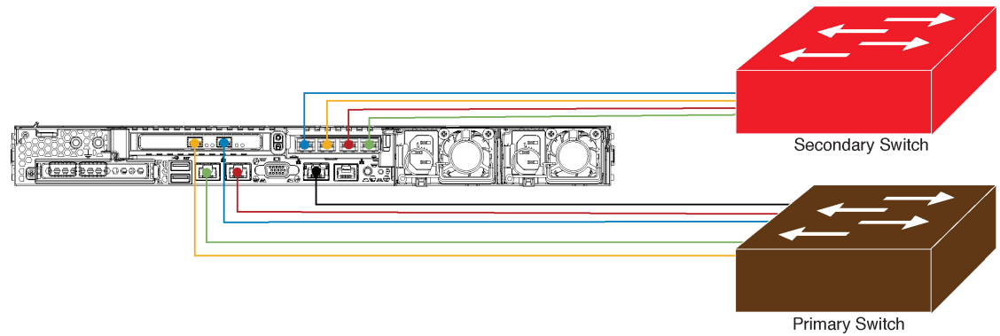
Figure 1: Recommended Cabling for 44 and 56-Core Appliance
