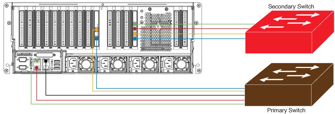
Figure 2: Recommended Cabling for 112-Core Appliance
