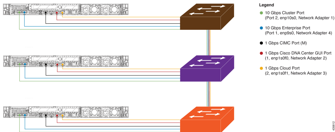
Figure 2: Recommended Cabling for Three-Node Cluster
