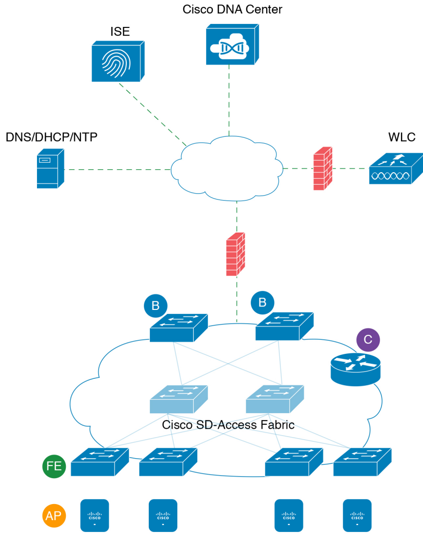
Figure 5: Cisco SD-Access Fabric Infrastructure
