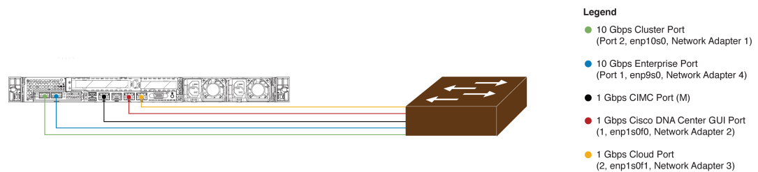
Figure 3: Recommended Cabling for Single-Node Cluster
