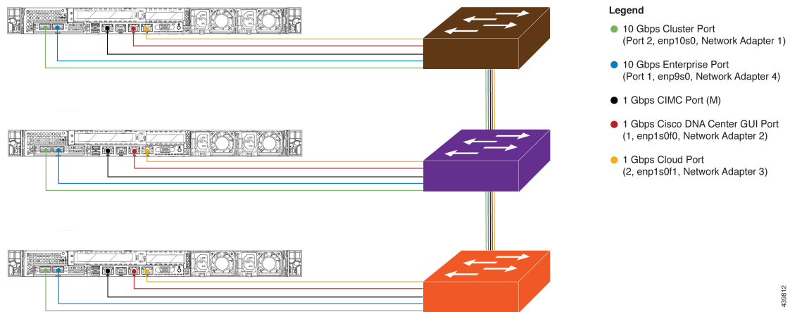
Figure 4: Recommended Cabling for Three-Node Cluster
