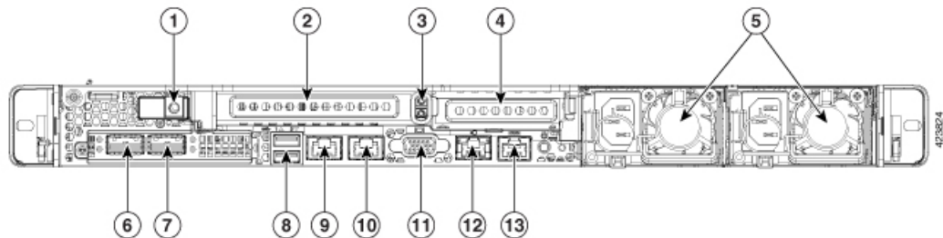
Figure 2: Appliance Rear Panel
