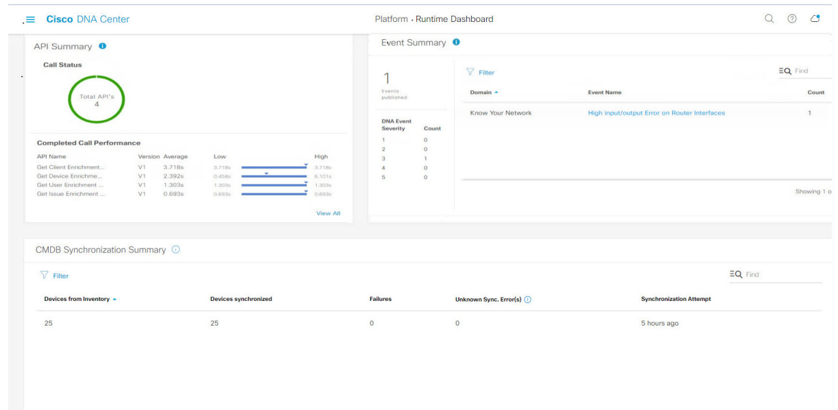
Figure 146: Cisco DNA Center Platform Runtime Dashboard Window
