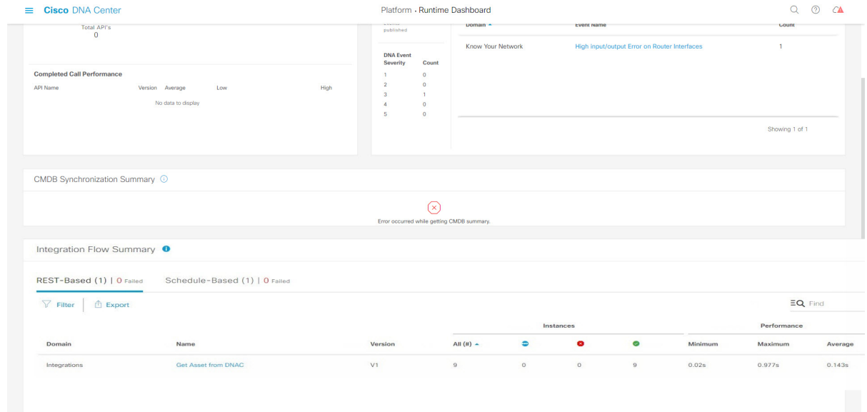
Figure 148: Cisco DNA Center Platform Runtime Dashboard Window
