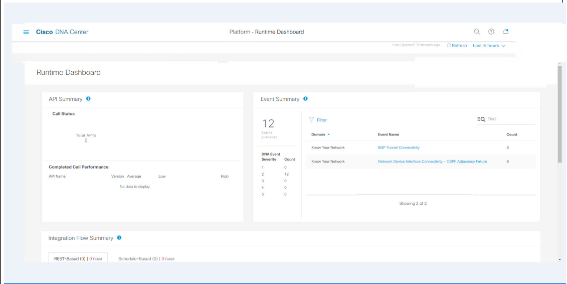
Figure 33: Event Summary
