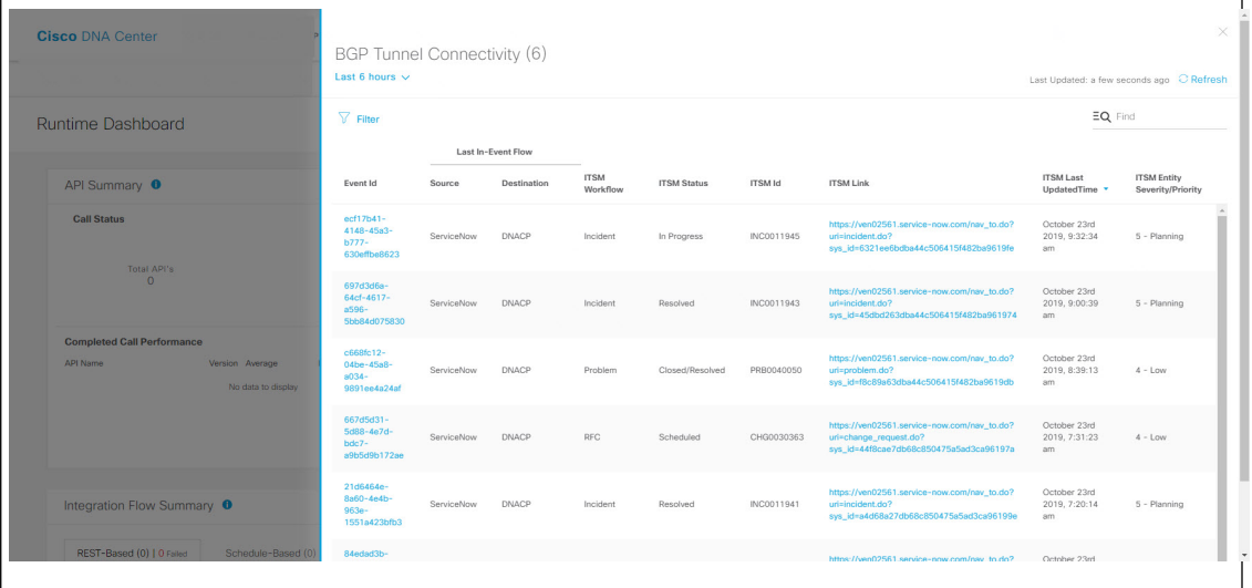
Figure 34: Event History
