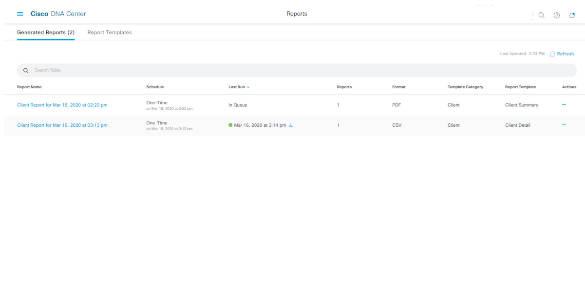
Figure 101: Generated Reports
