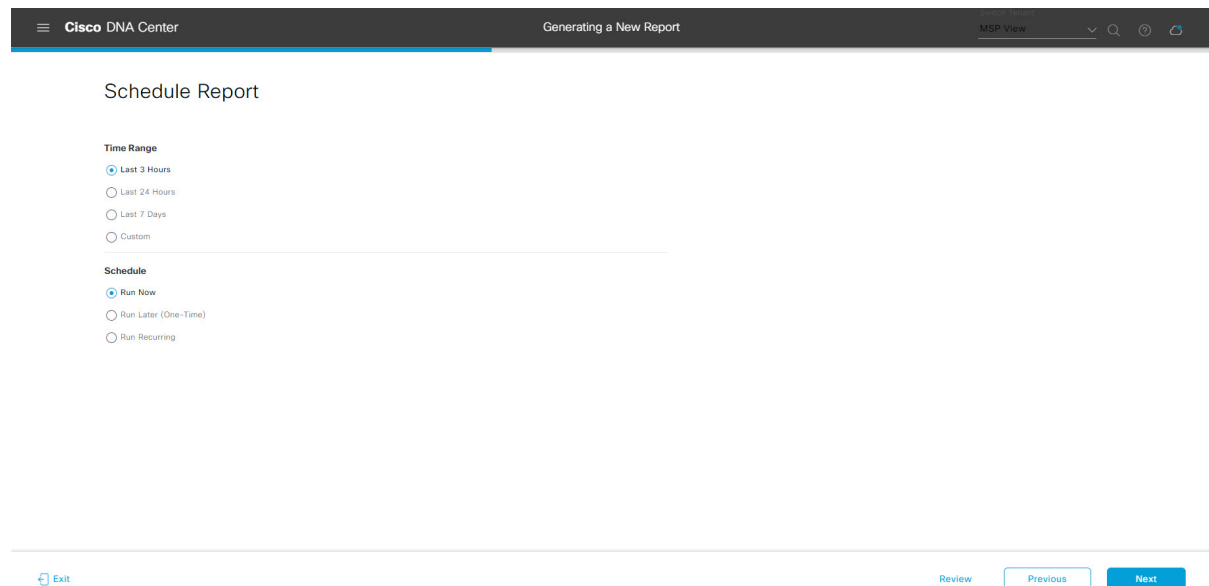
Figure 98: Schedule Report
