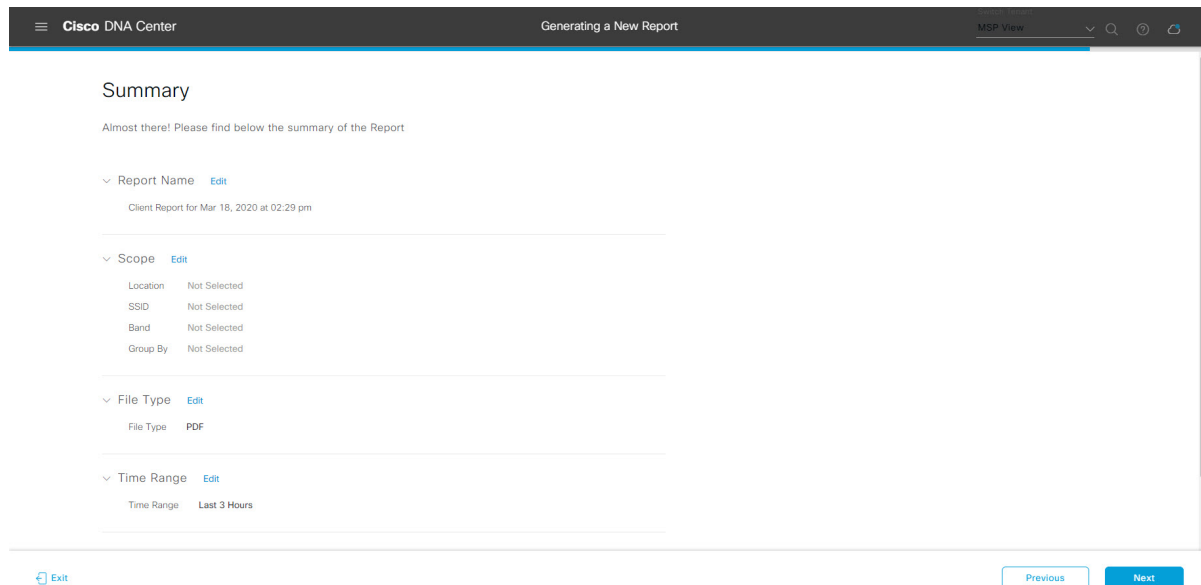
Figure 100: Summary
