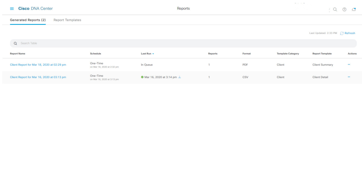
Figure 31: Generated Reports
