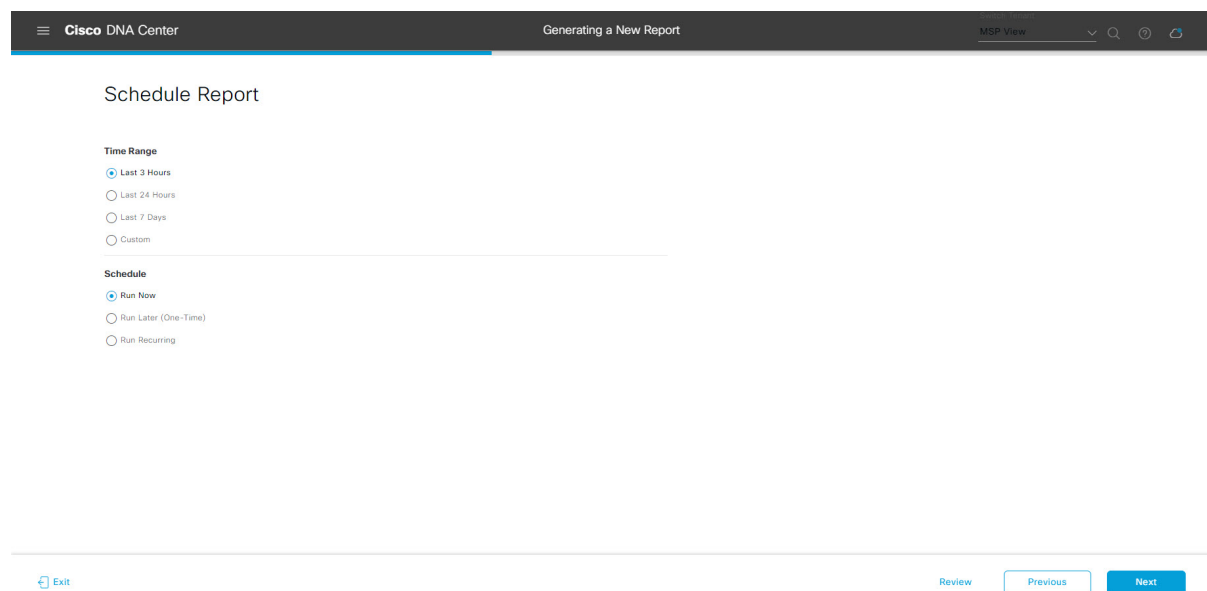
Figure 8: Schedule Report
