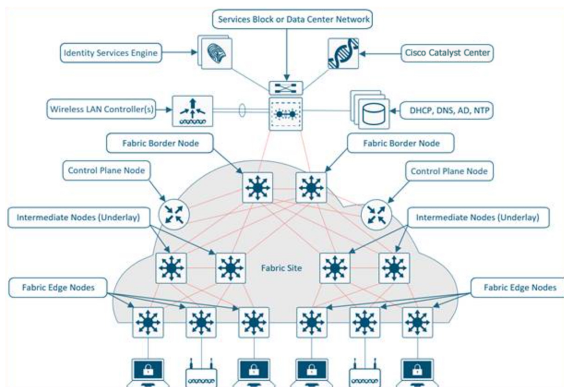
Figure 7: Cisco SD-Access fabric infrastructure
