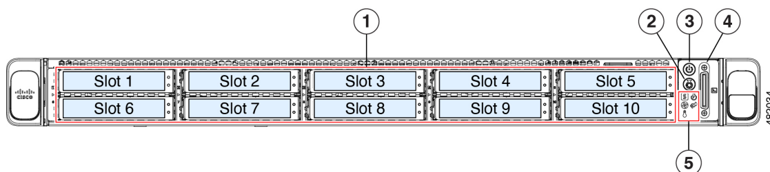
Figure 1: Front panel
