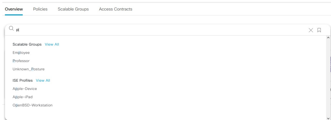
Figure 4: Search Window
