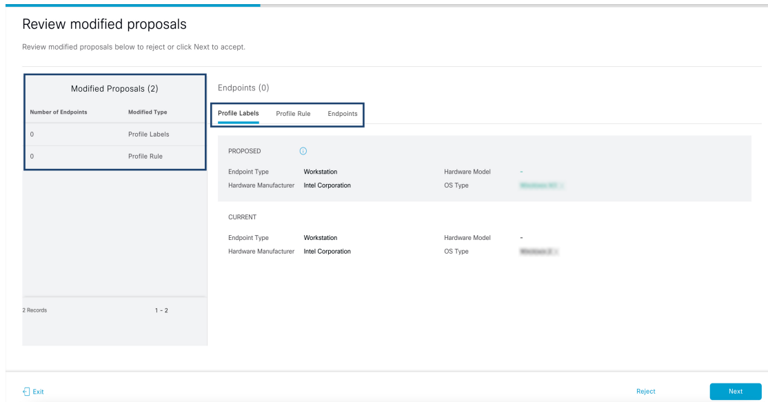
Figure 11: Review Modified Proposals Window of the Review AI Proposals Workflow
