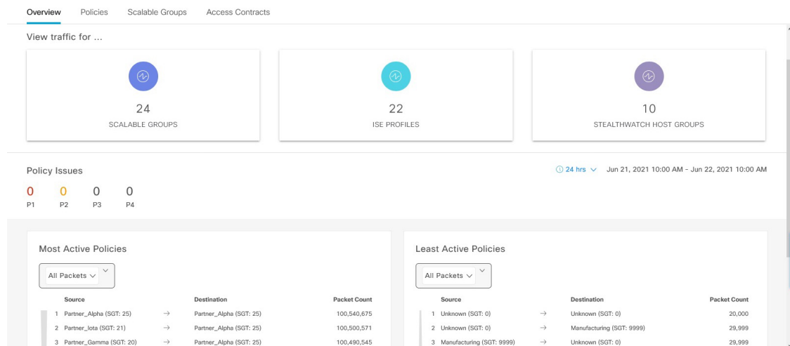
Figure 23: Group-Based Access Control Policy Dashboard
