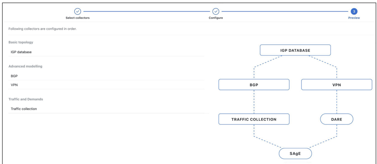
Figure 12: Preview Page
