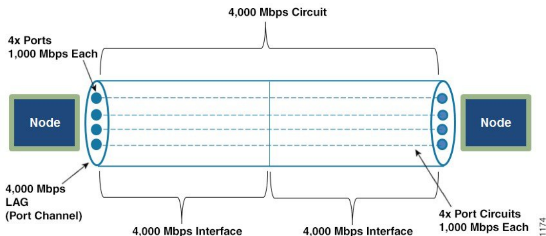
Figure 1: Ports, Port Circuits, and LAGs
