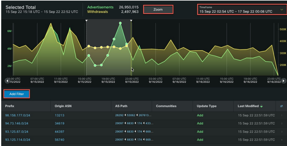
Figure 1: BGP Updates Page
