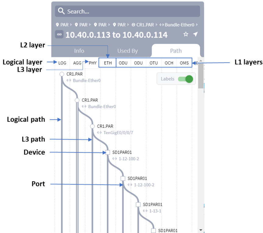
Figure 30. Example of the Layers in a Path of a Logical Link.
