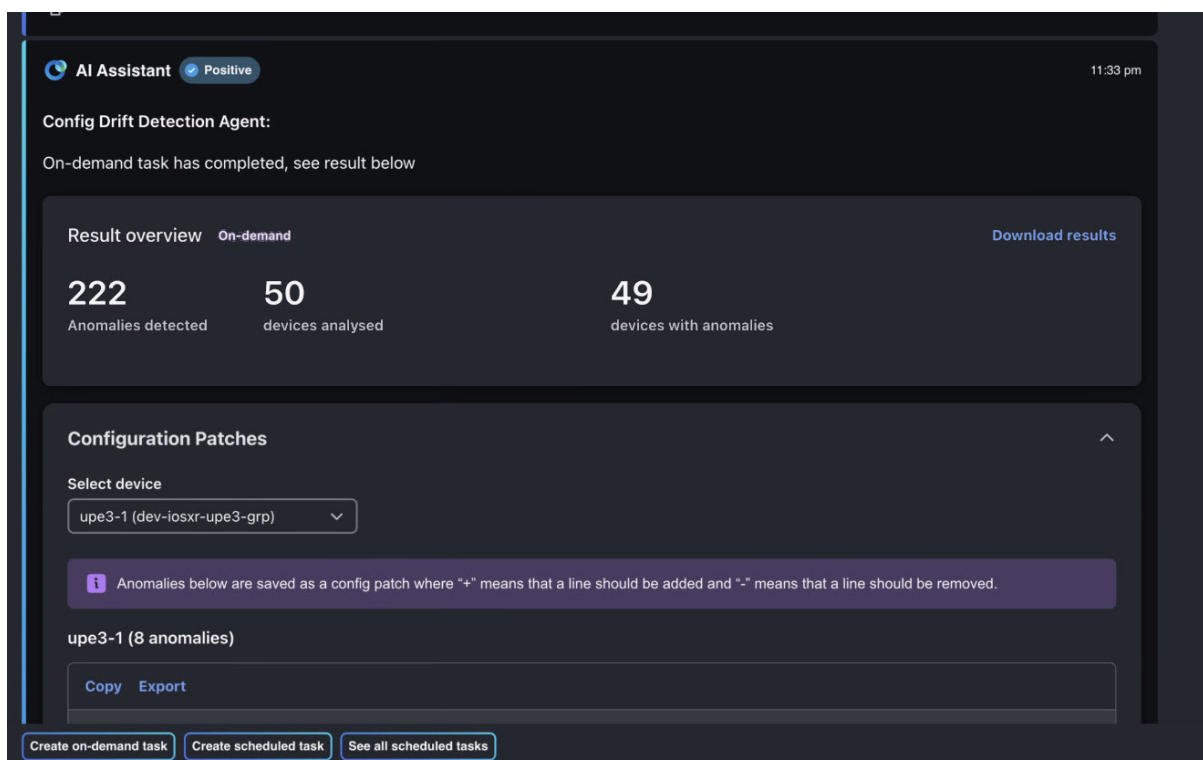
Figure 9. CDD inference result
