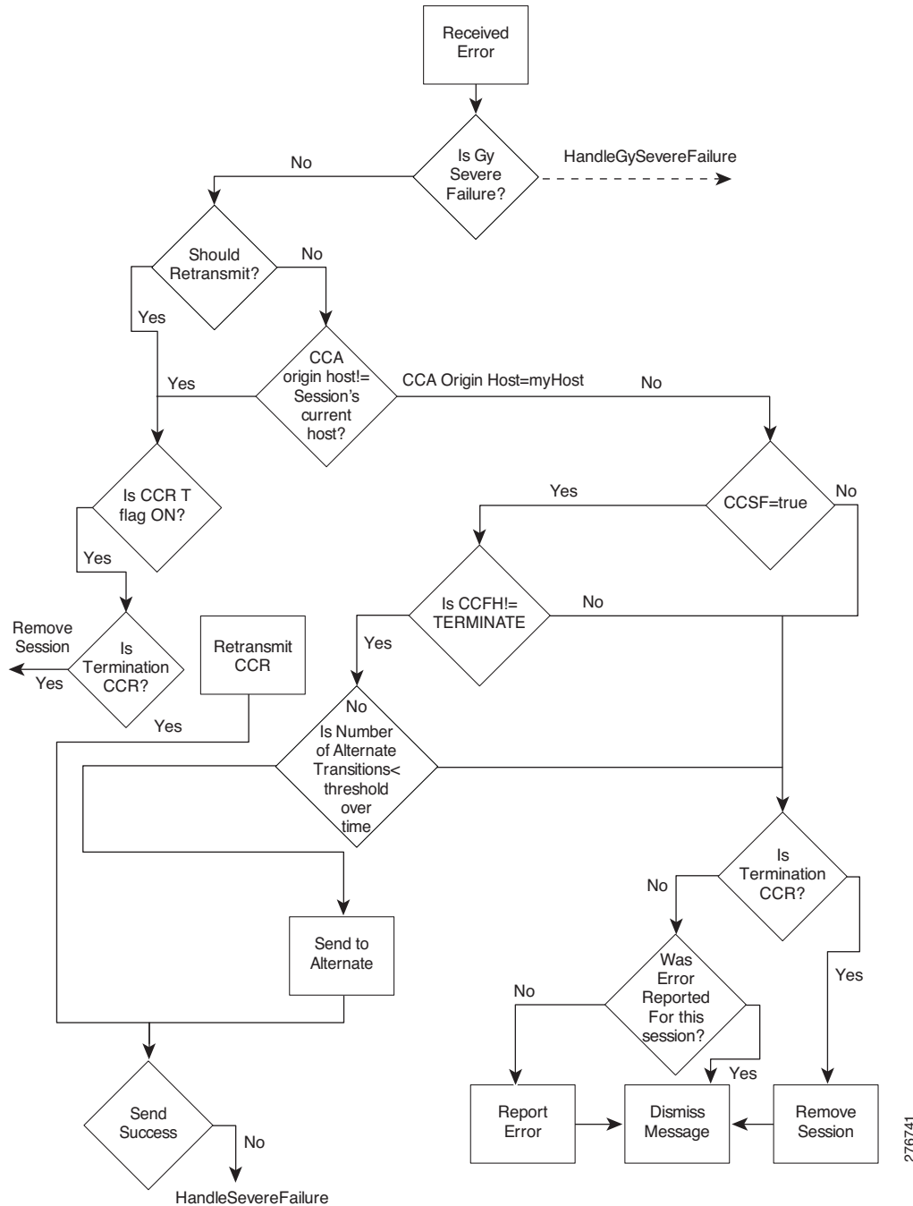
Figure 1-19 Gy Client Behavior Upon CCA Error or Timeout Error
