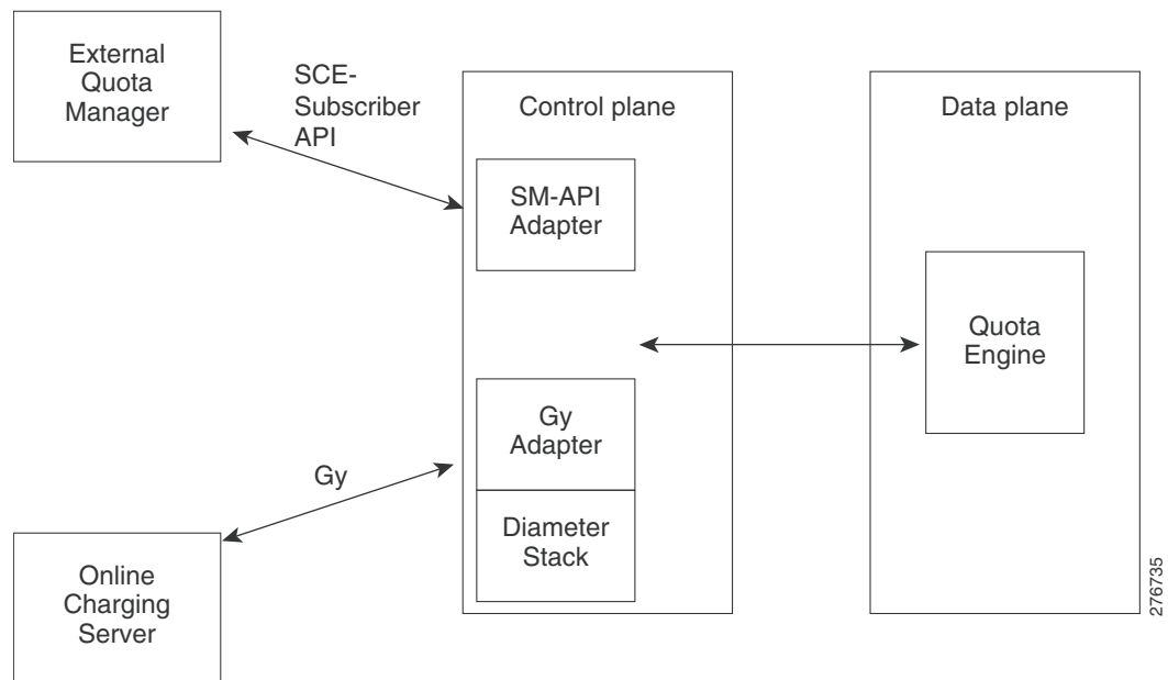
Figure 1-1 Gy Interface Adapter
