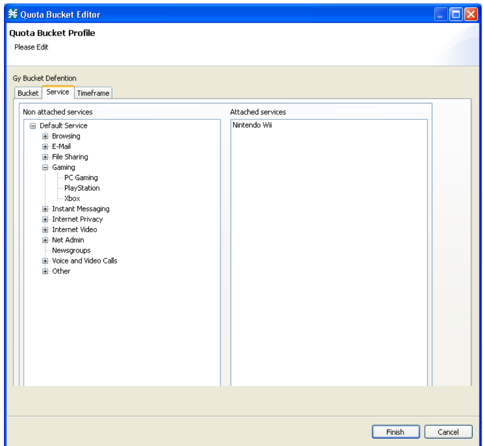
Figure 1-13 Quota Bucket Editor - Service Tab
