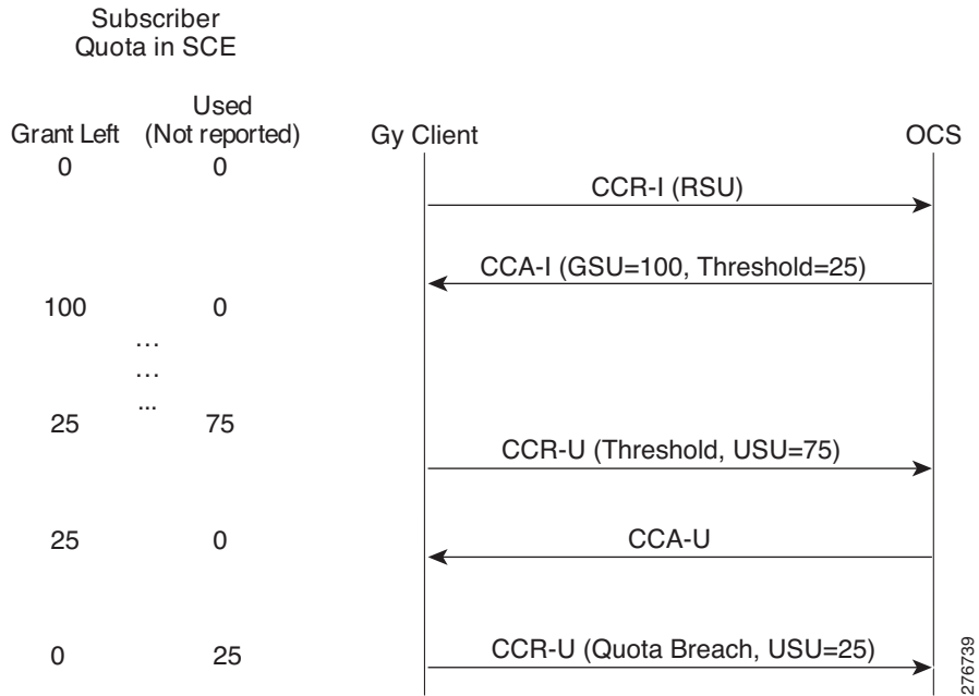
Figure 1-5 Gy Quota Threshold Call Flow
