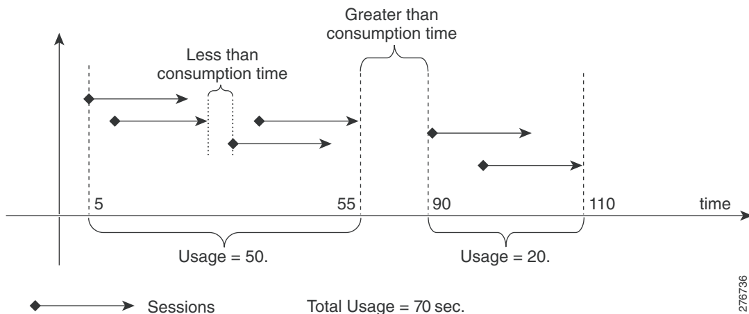
Figure 1-2 Quota Consumption Time
