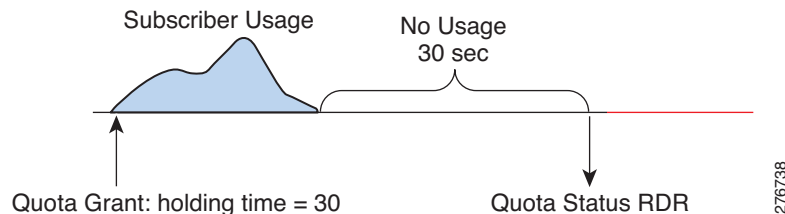
Figure 1-4 Quota Holding Time
