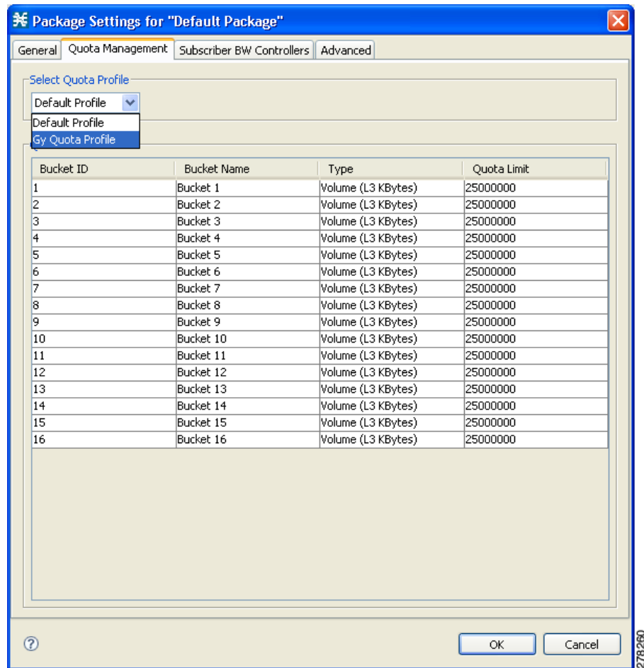
Figure 1-15 Package Settings – Quota Management Tab
