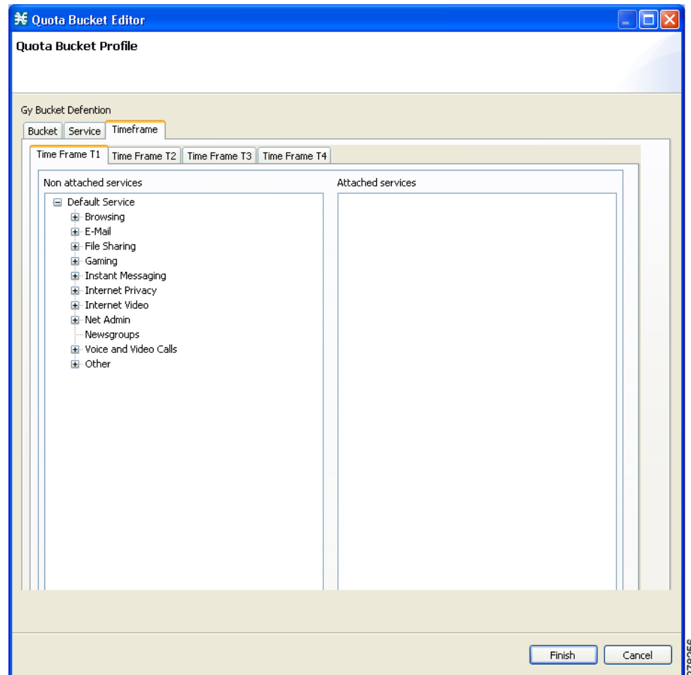
Figure 1-14 Quota Bucket Editor - Timeframe Tab
