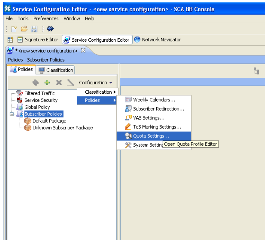
Figure 1-6 Accessing the Quota Profile Editor
