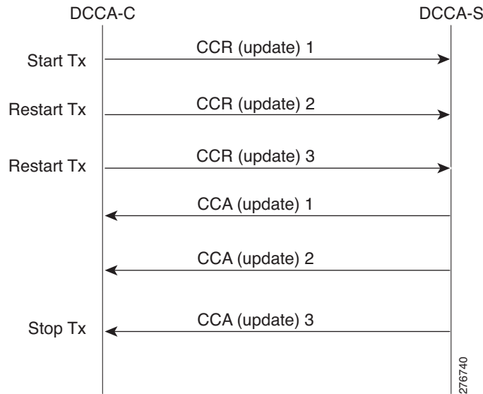
Figure 1-18 Tx Timer Behavior
