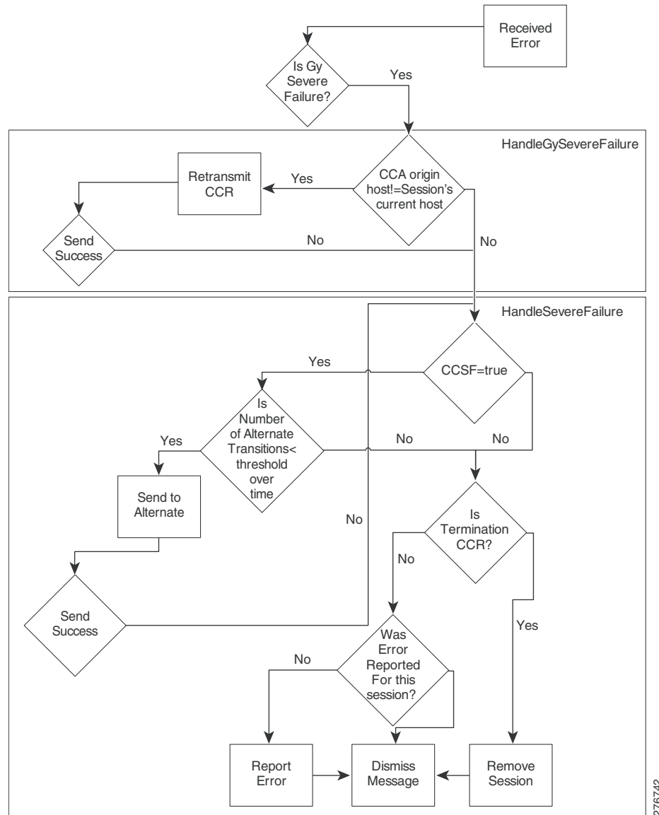
Figure 1-20 Gy Client Behavior Upon Severe Failure
