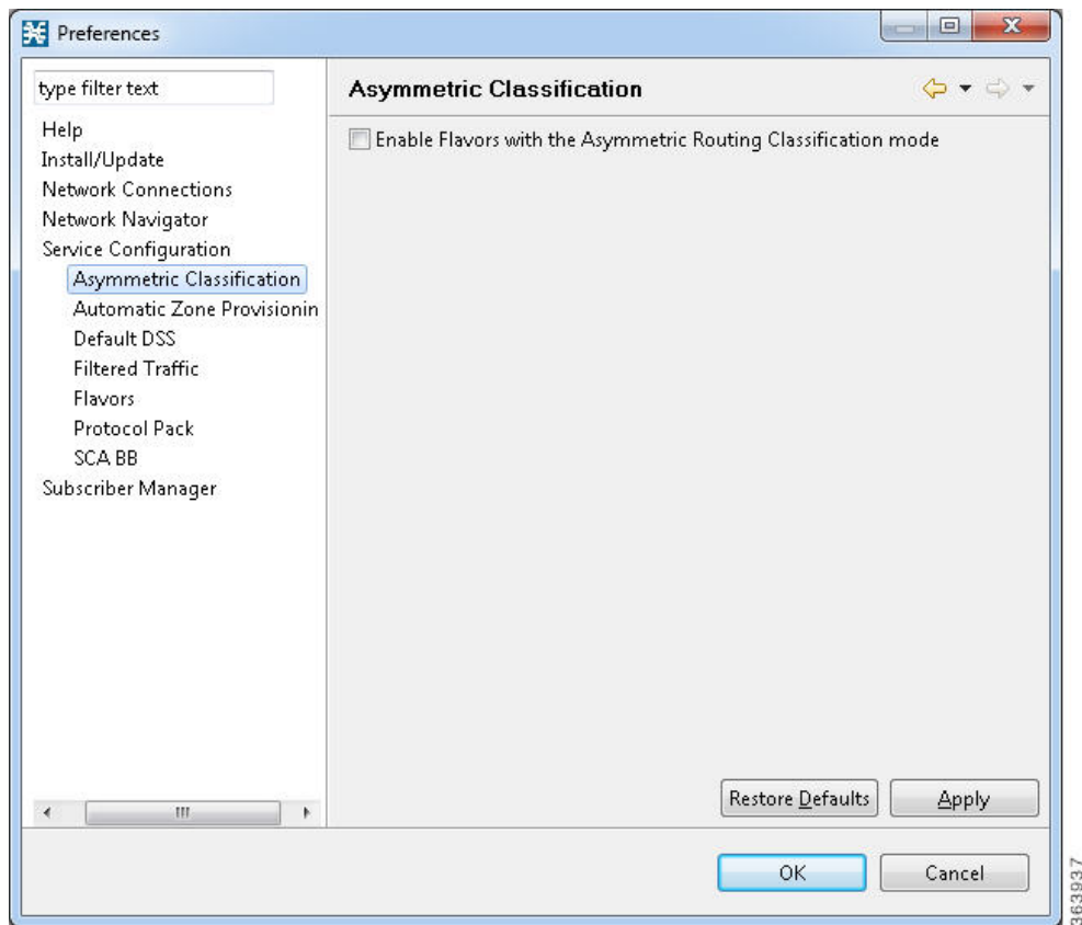
Figure 45: Asymmetric Classification - Preferences
