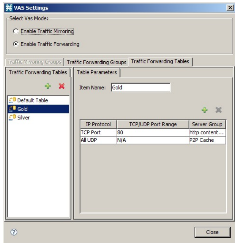
Figure 52: Traffic Forwarding Tables Tab
