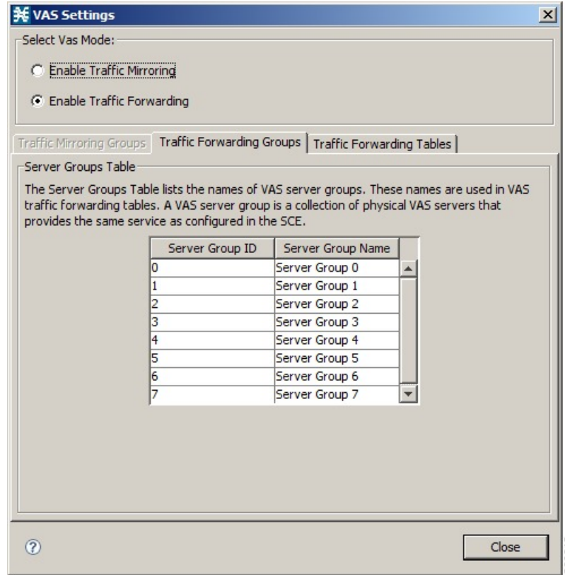
Figure 48: VAS Settings - Enable Traffic Forwarding
