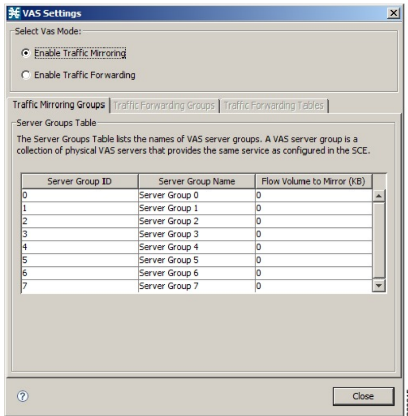
Figure 49: VAS Settings - Enable Traffic Mirroring
