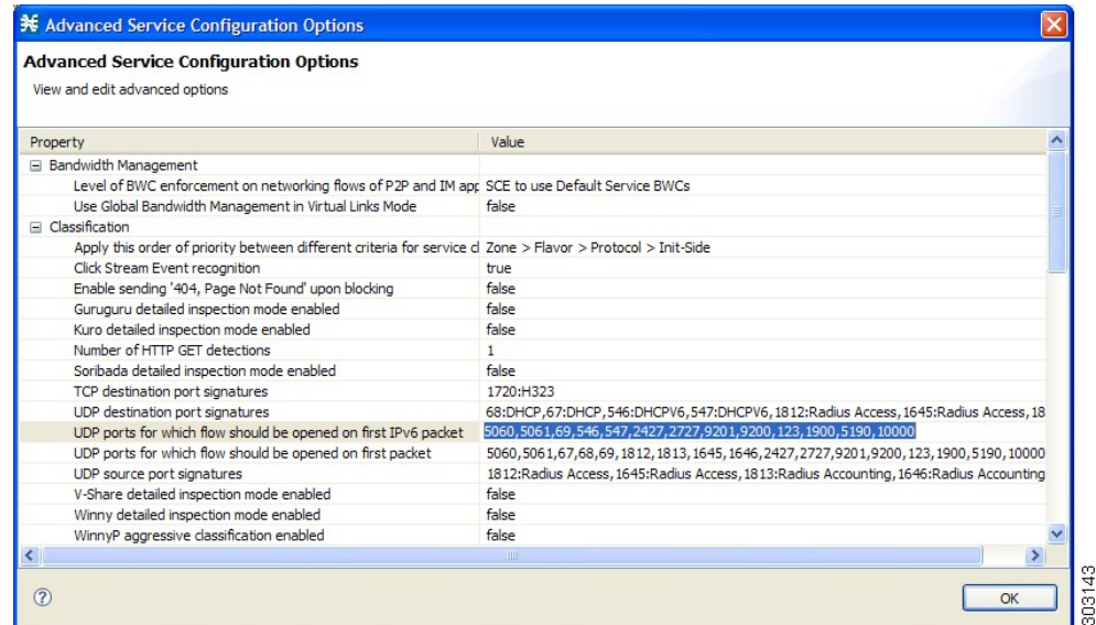
Figure 47: Advanced Service Configuration Options
