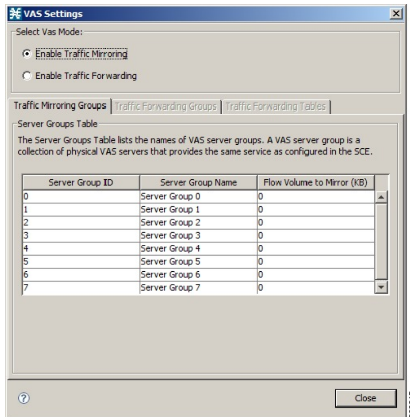
Figure 51: Traffic Mirroring Groups Tab
