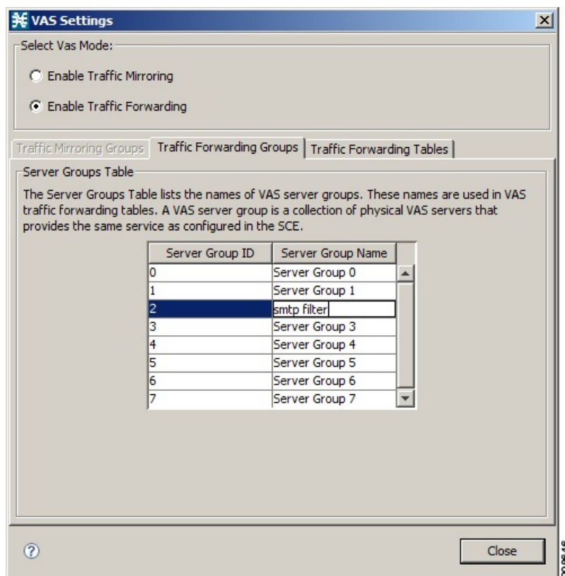
Figure 50: Traffic Forwarding Groups Tab
