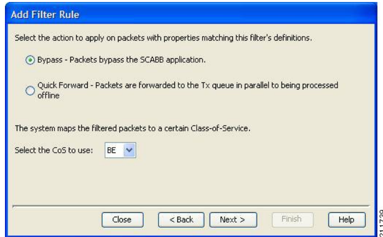
Figure 22: Action and Class-of-Service
