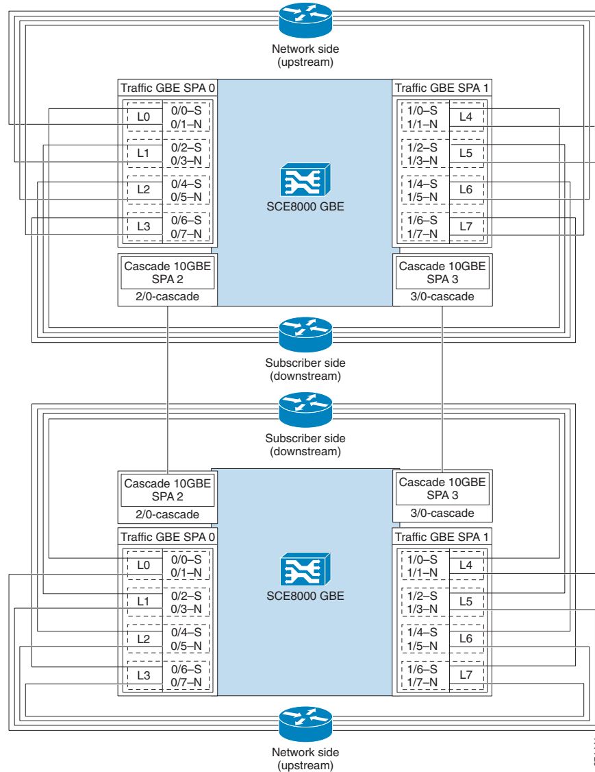
Figure 11-1 In-line Dual-Platform Redundant Topology
