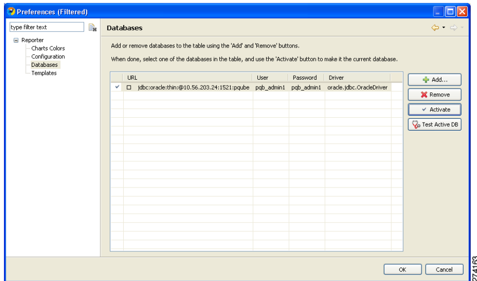
Figure 2-16 Preferences (Filtered)—Databases
