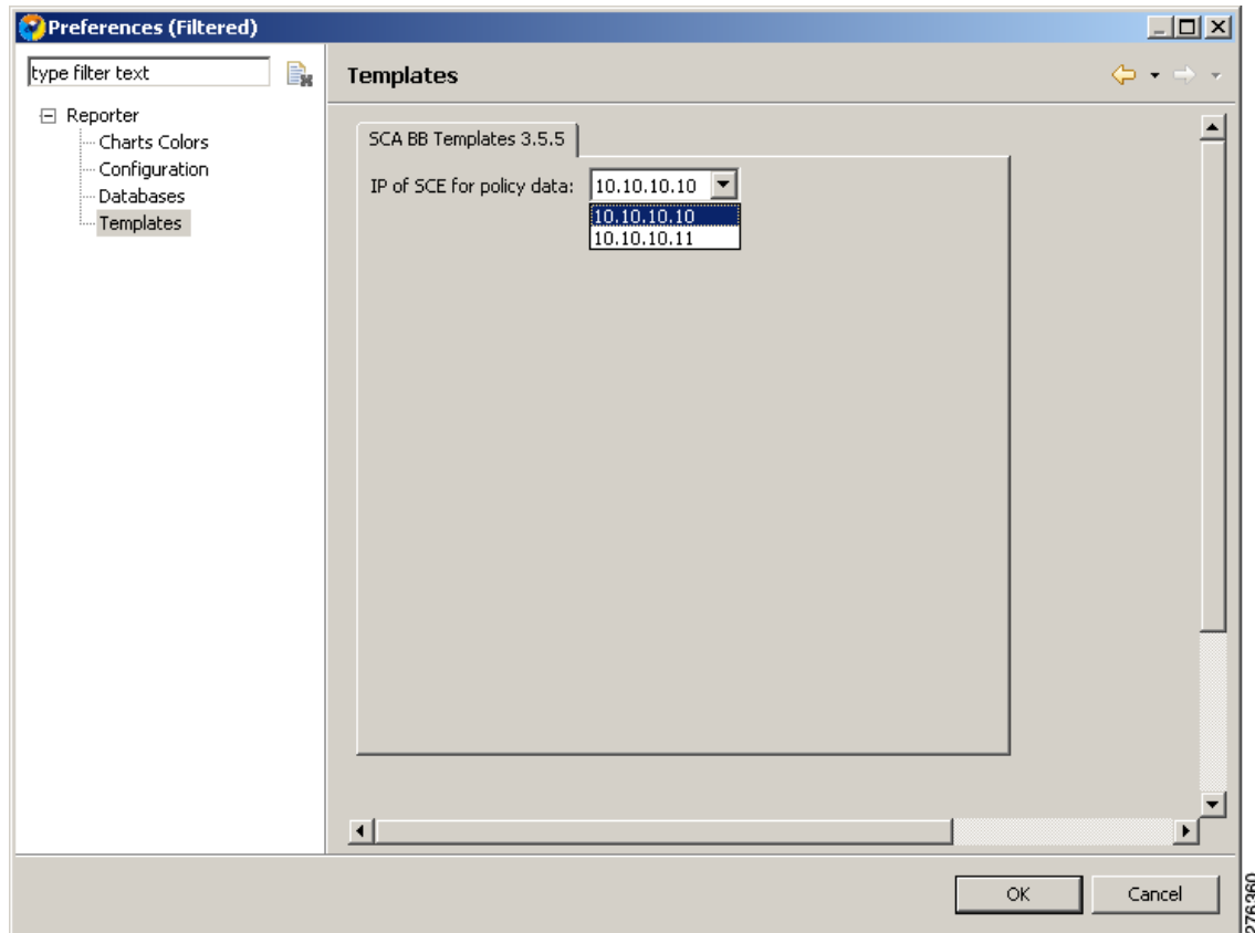
Figure 2-17 Preferences (Filtered)—Templates
