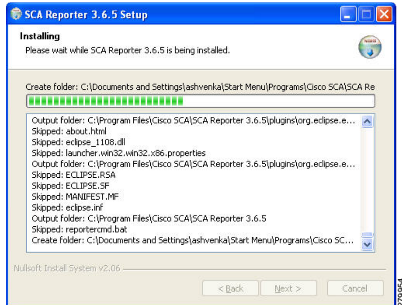
Figure 2-4 Installing
