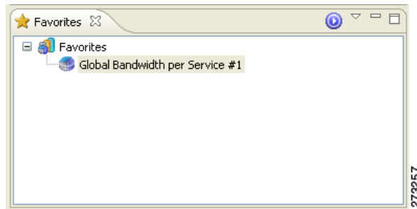
Figure 2-34 Favorites
