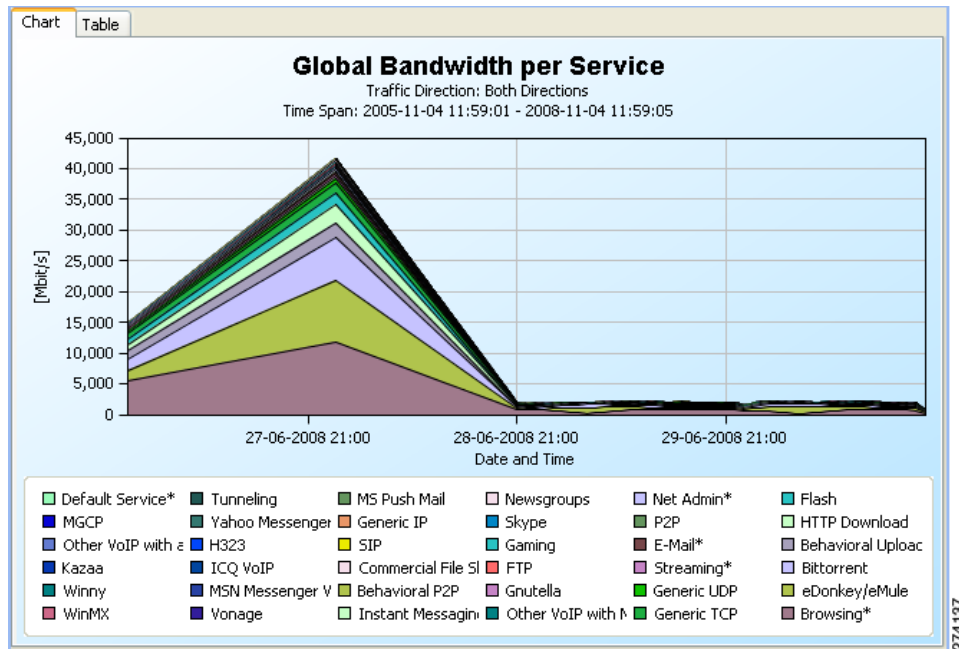
Figure 2-35 Report
