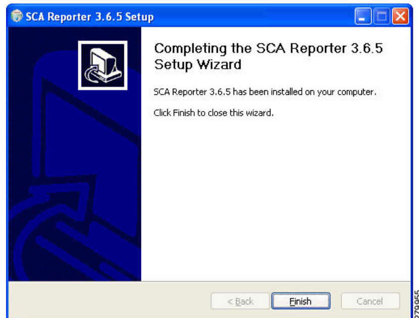
Figure 2-5 Installation Complete
