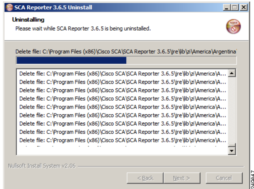
Figure 2-8 Uninstall
