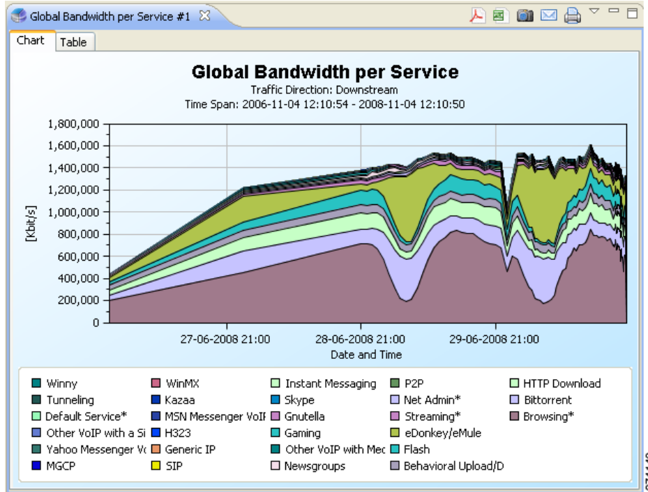
Figure 2-40 Modified Report
