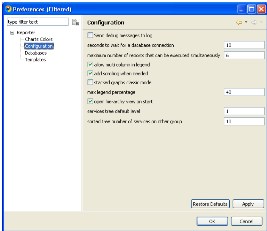
Figure 2-24 Preferences (Filtered)—Configuration
