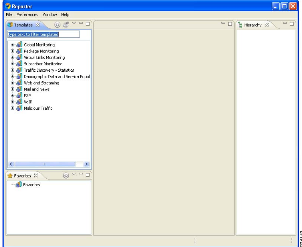
Figure 2-28 Reporter
