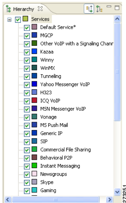
Figure 2-36 Hierarchy
