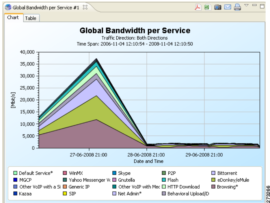
Figure 2-38 Modified Report
