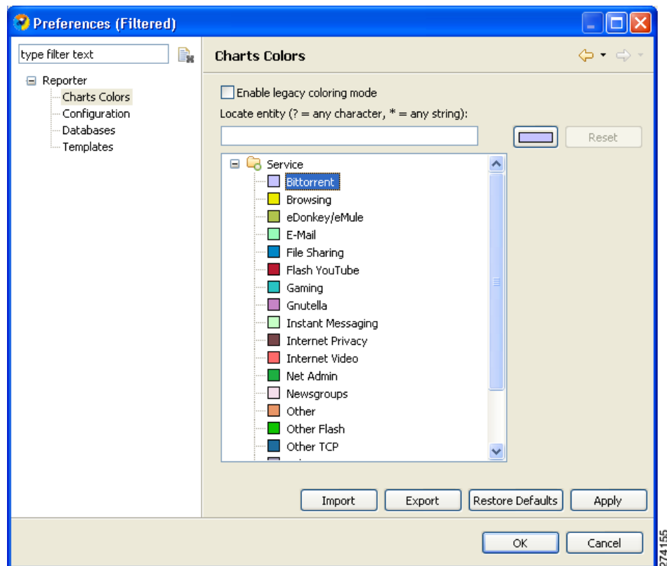
Figure 2-21 Current Color
