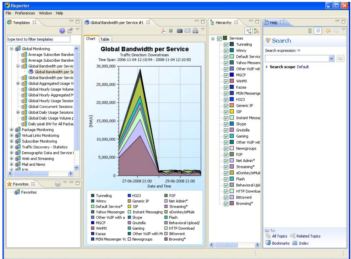
Figure 2-27 Reporter Help
