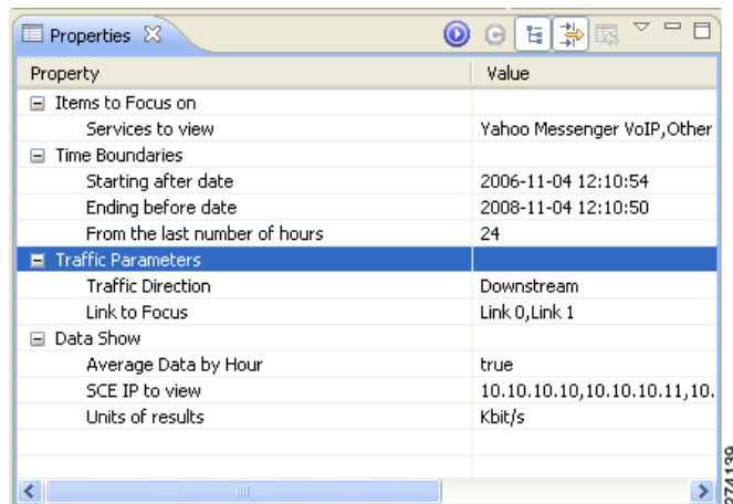
Figure 2-39 Report Properties
