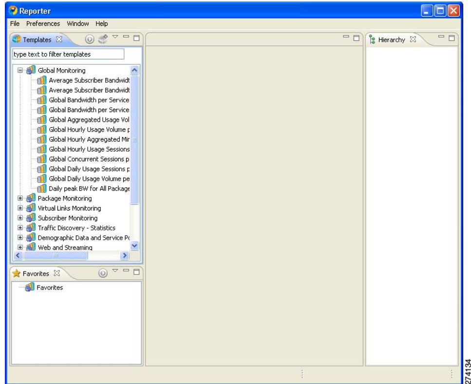
Figure 2-29 Templates
