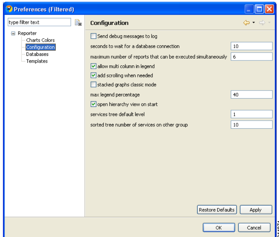
Figure 2-25 Preferences (Filtered)—Configuration
