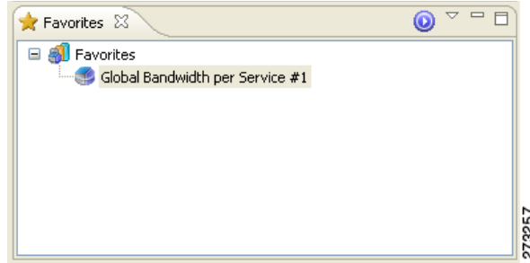
Figure 4-8 Favorites
