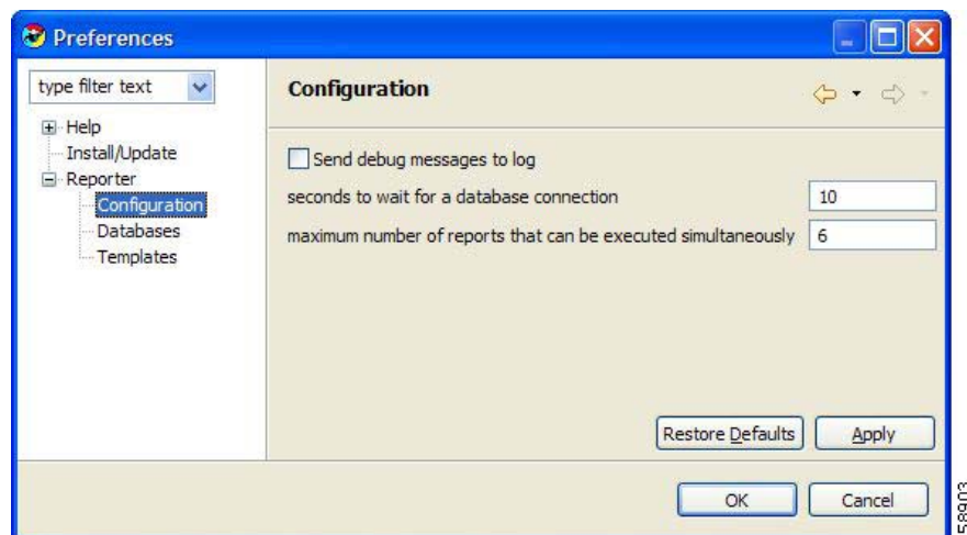
Figure 2-26 Preferences (Filtered)—Configuration
