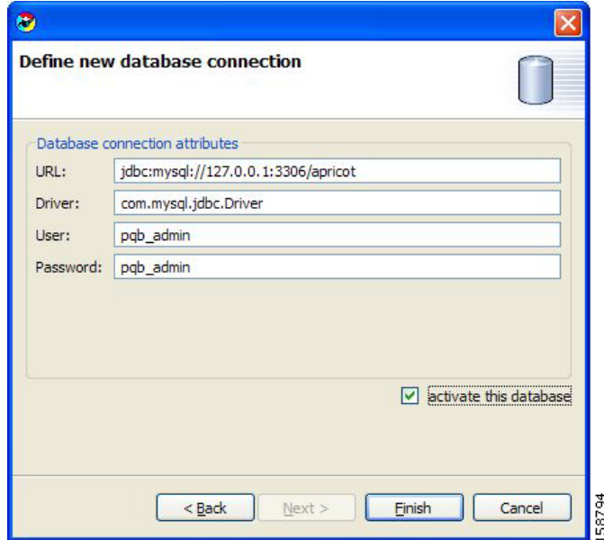
Figure 2-15 Advanced Definition
