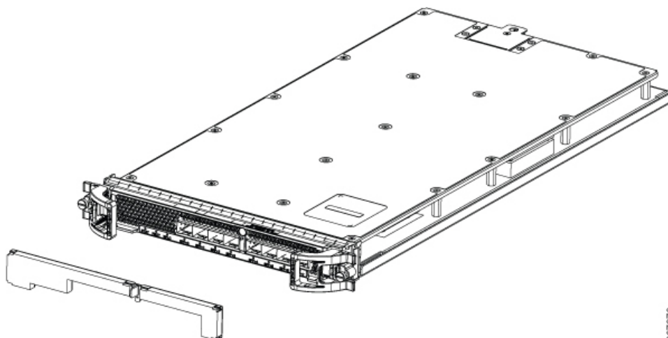
Figure 13: Air Filter
