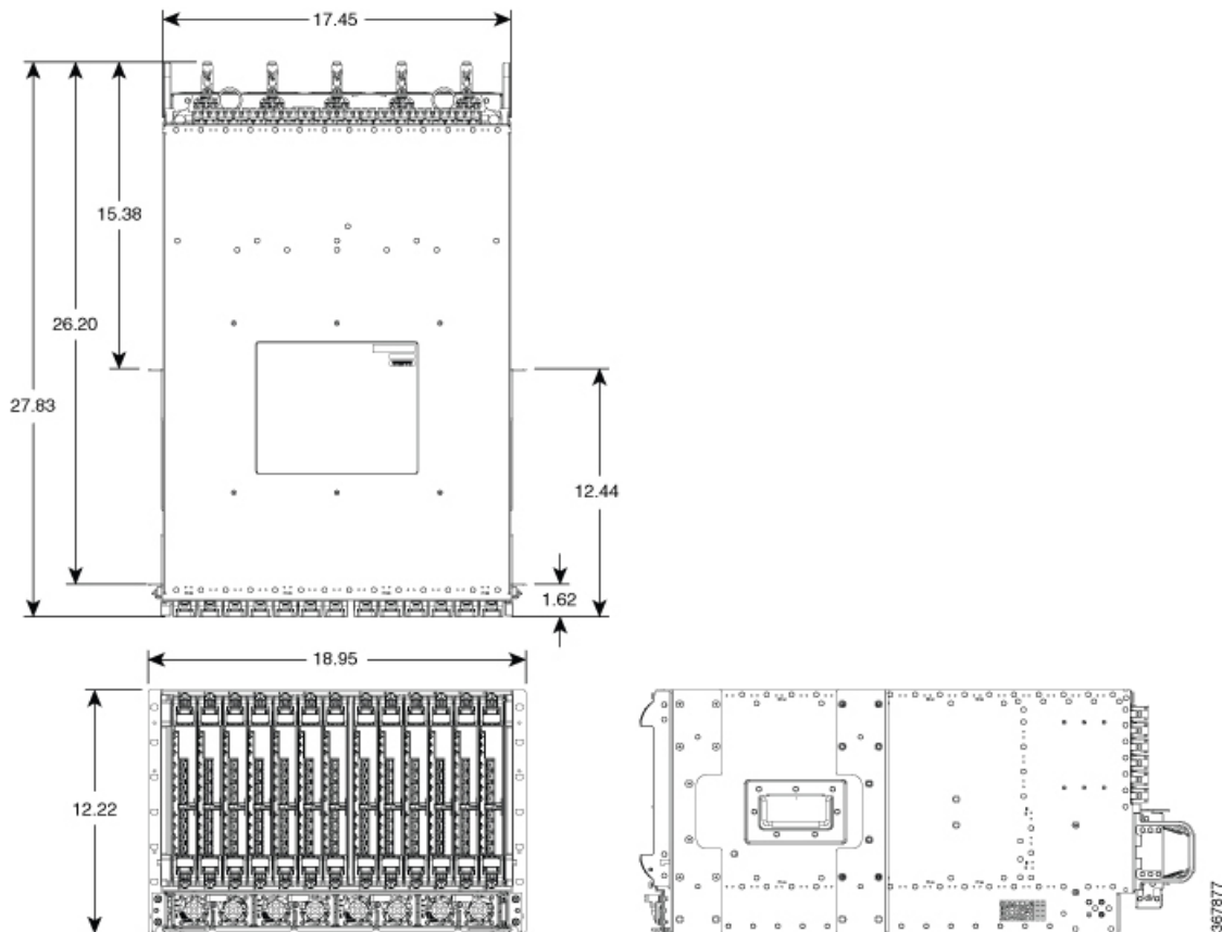
Figure 2: Cisco Remote PHY Shelf 7200 dimensions
