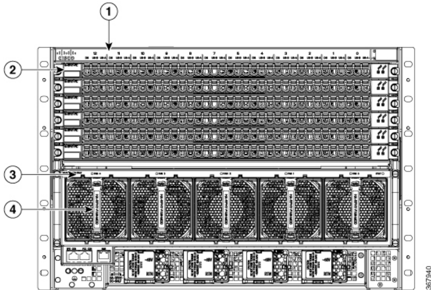
Figure 4: Cisco Remote PHY Shelf 7200 Rear View
