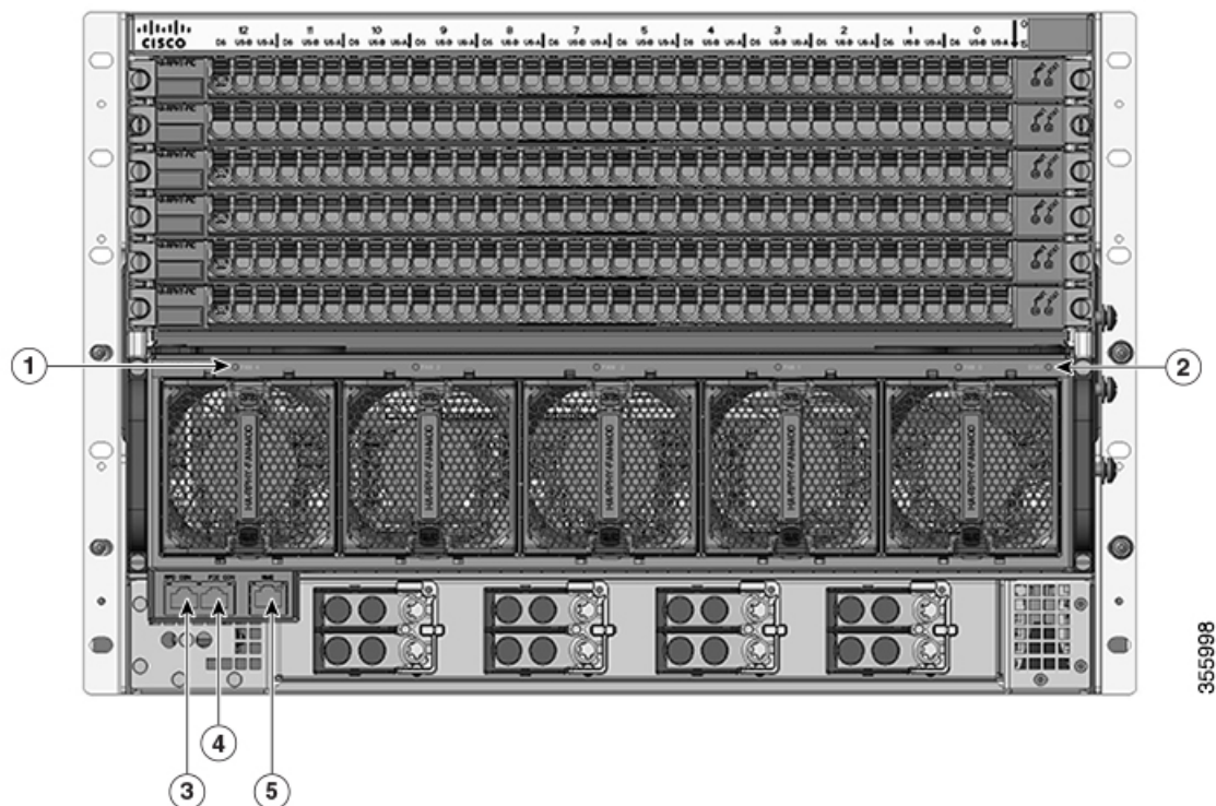
Figure 5: Cisco Remote PHY Shelf 7200 LED's and ports
