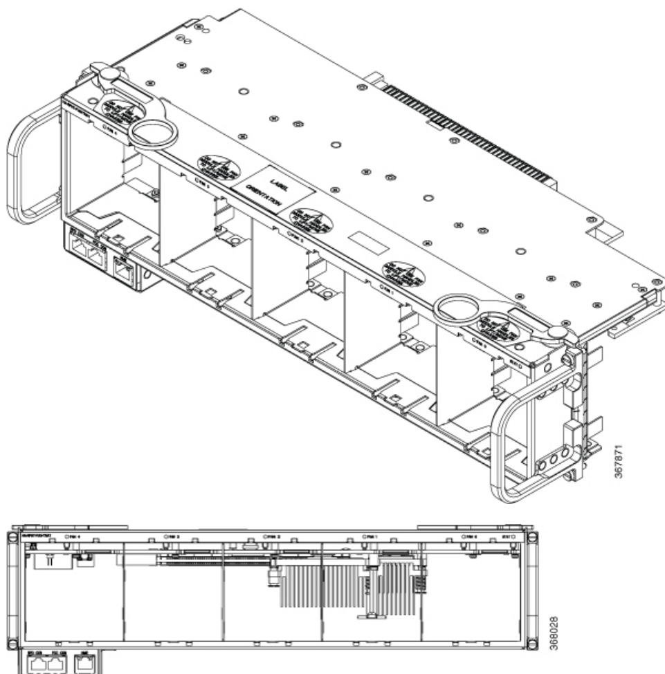
Figure 8: An empty Fan Tray
