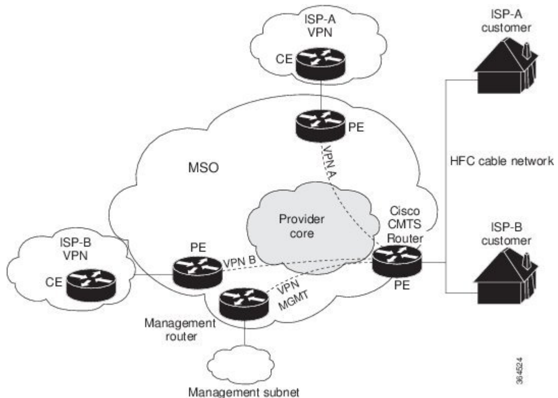
Figure 3: MPLS VPN Network
