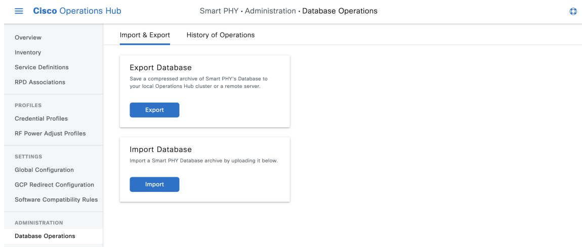
Figure 1: Database Operations
