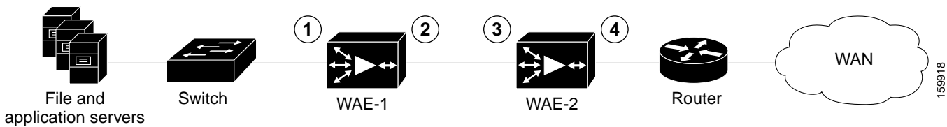
Figure 5-9 Inline Cluster
