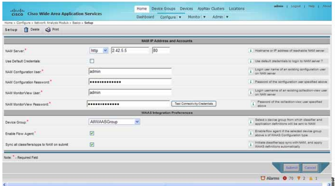
Figure 13-1 Setup Window
