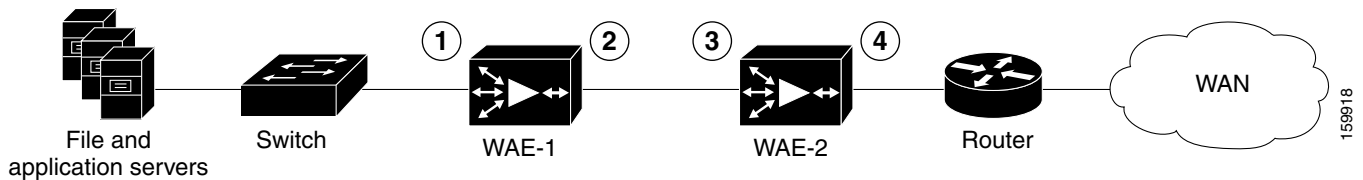
Figure 4-10 Inline Cluster
