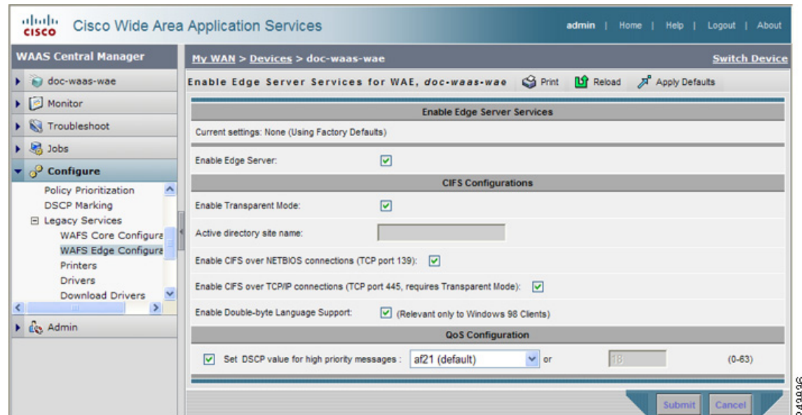
Figure 11-4 Enabling File Services on Edge Devices
