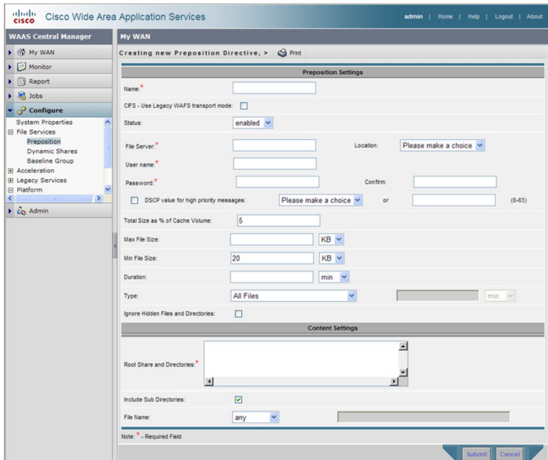
Figure 11-6 Creating a New Preposition Directive
