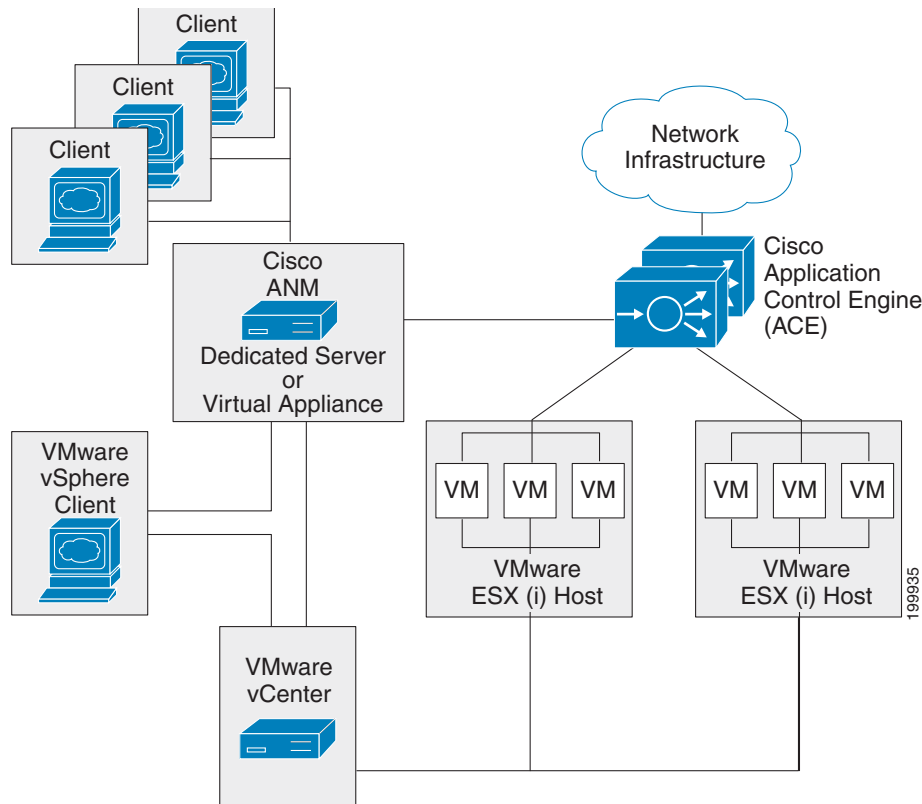
Figure 22-1 ANM Integrated With VMware vCenter Server and vSphere Client
