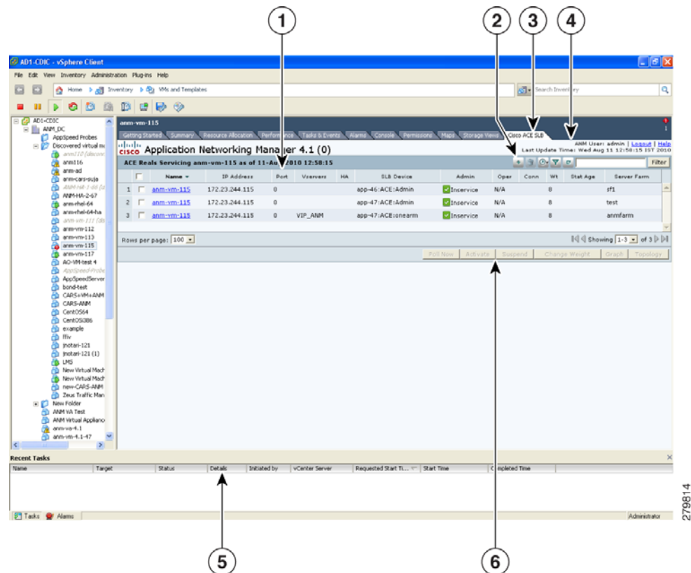
Figure 22-2 Cisco ACE SLB Tab in vSphere Client
