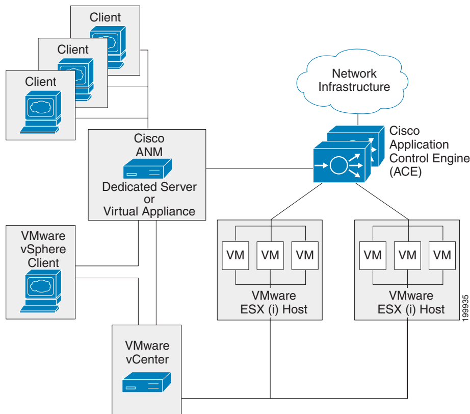
Figure 1-1 Sample ANM Network Deployment
