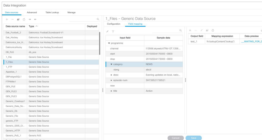
Figure 36 Paste XML into Sample Data Panel
