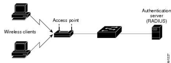
Figure 29: Multiple Host Mode Example
