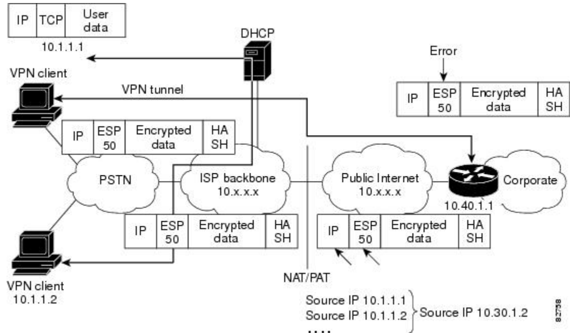
Figure 48: Standard IPsec Tunnel Through a NAT/PAT Point (No UDP Encapsulation)
