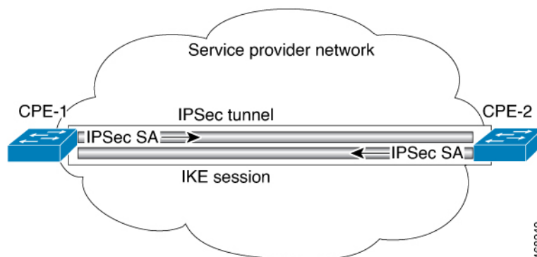
Figure 44: IPsec Tunnel
