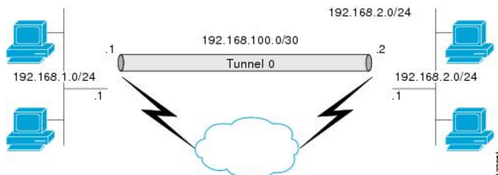
Figure 45: IPsec SVTI
