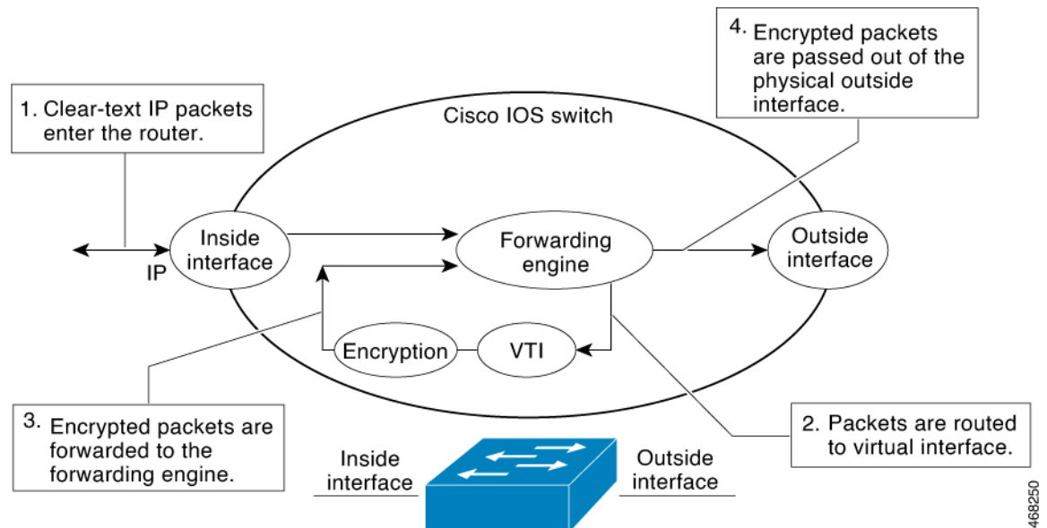
Figure 46: Packet Flow into the IPsec Tunnel
