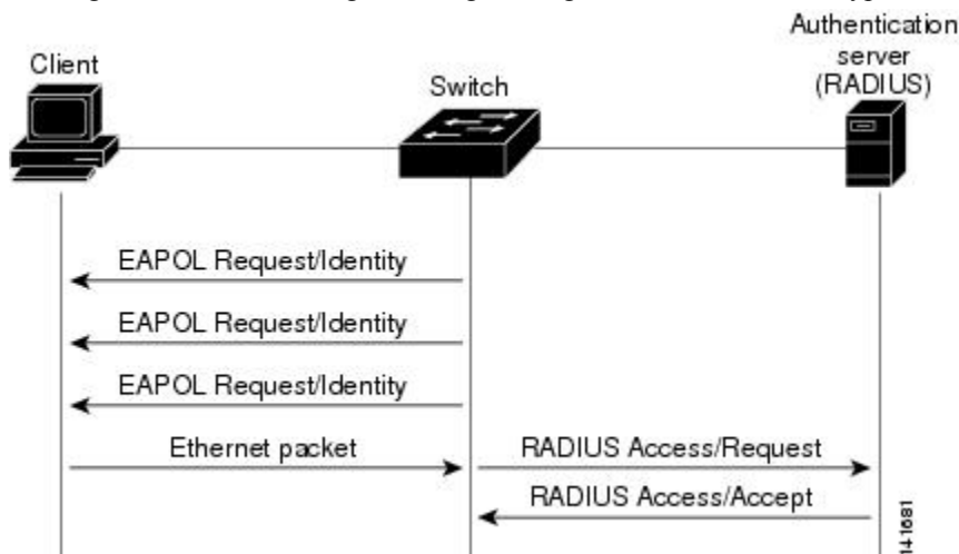
Figure 28: Message Exchange During MAC Authentication Bypass
