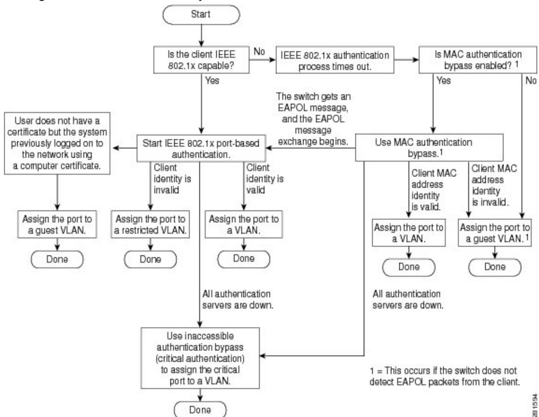
Figure 26: Authentication Flowchart
