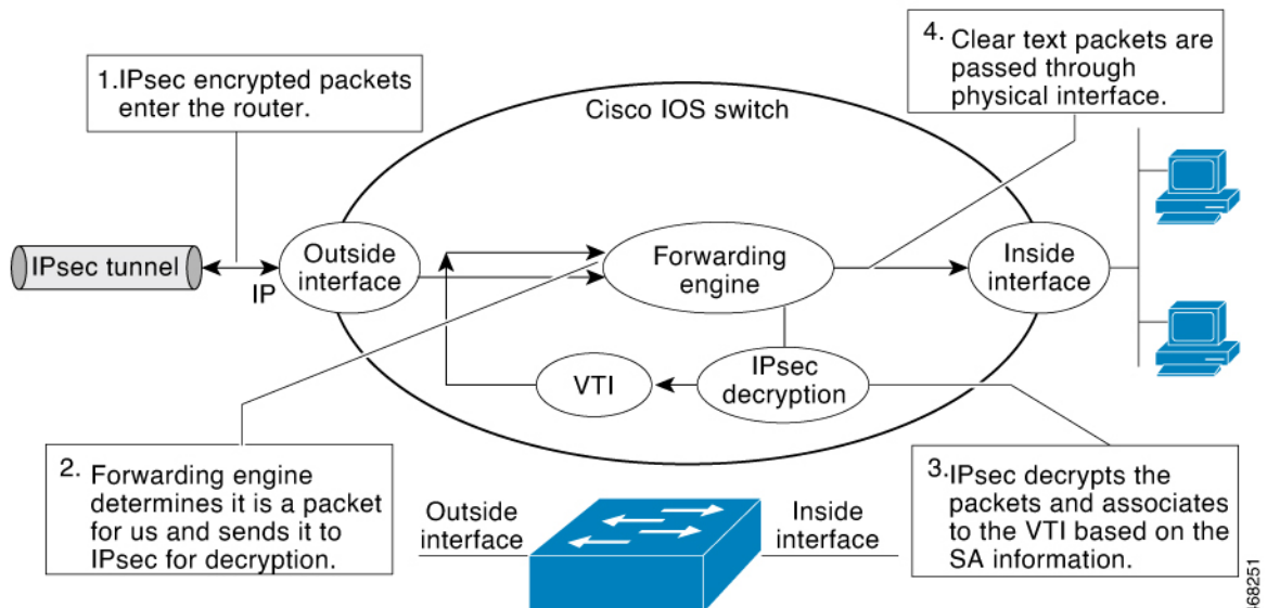
Figure 47: Packet Flow out of the IPsec Tunnel
