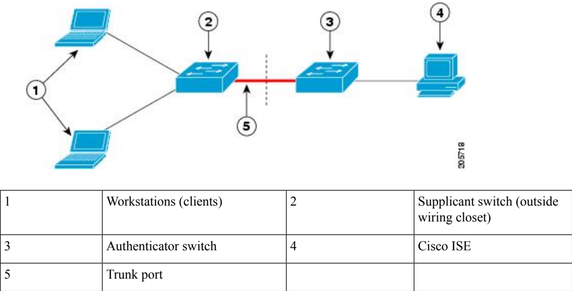
Figure 30: Authenticator and Supplicant Switch Using CISP
