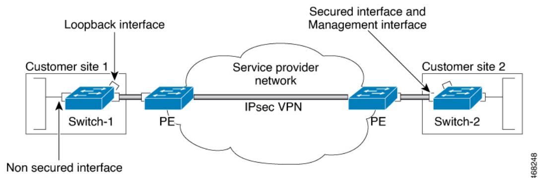
Figure 43: IPsec Network
