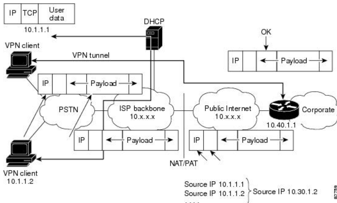
Figure 49: IPsec Packet with UDP Encapsulation
