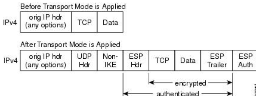
Figure 50: Transport Mode--IPsec Packet Before and After ESP Encapsulation
