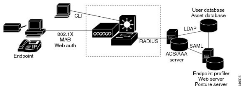
Figure 36: Sample Deployment of Cisco IBNS
