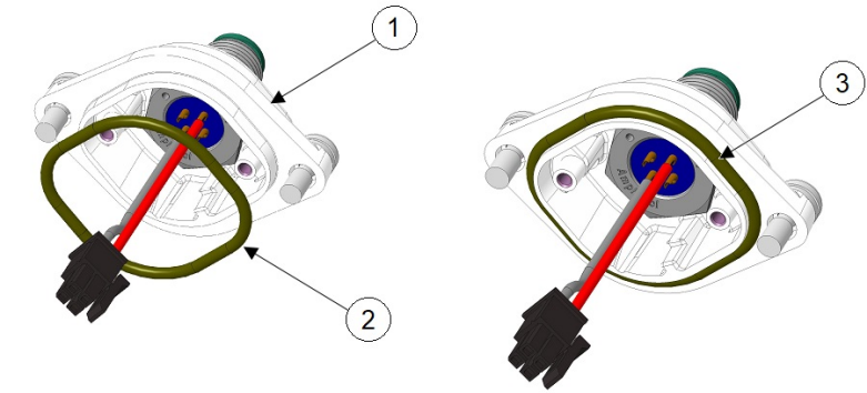
Figure 10: Installing O-ring on the M12 Adapter
