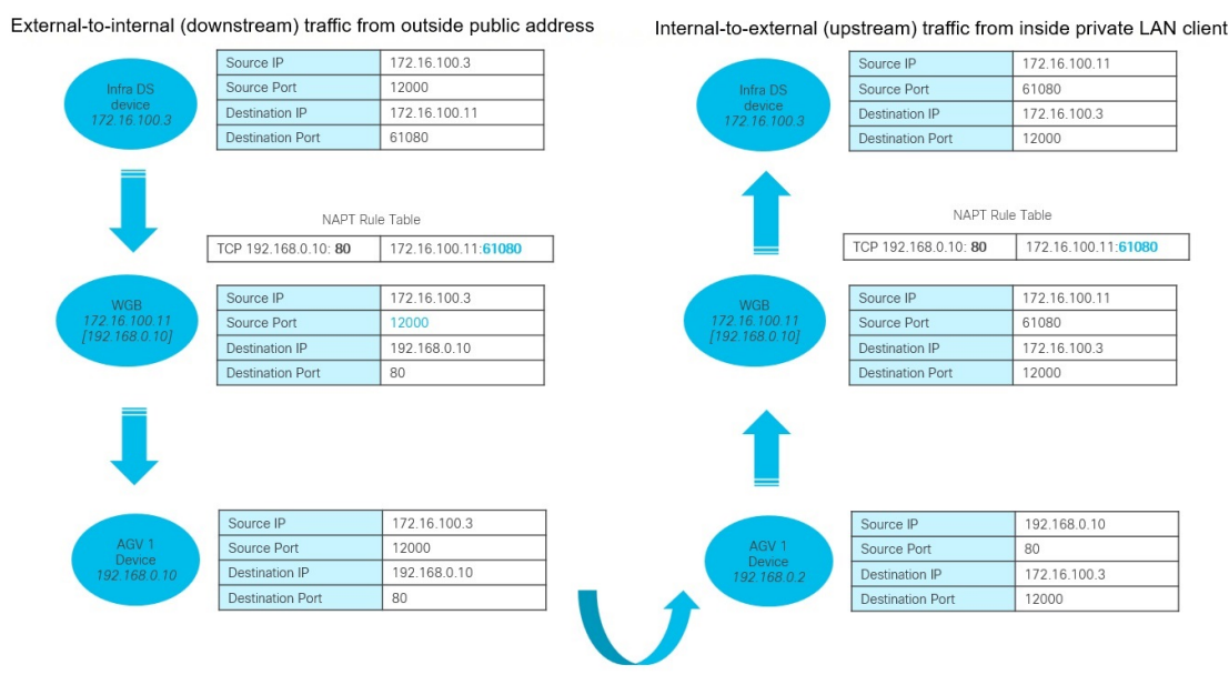
Figure 9: Upstream and downstream data flow using NAPT in uWGB
