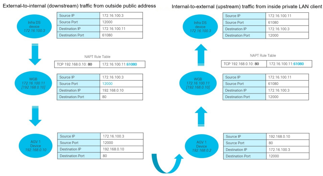
Figure 6: Upstream and downstream data flow using NATP in uWGB
