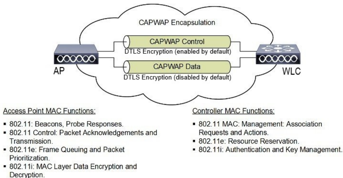
Figure 8: Split MAC Architecture
