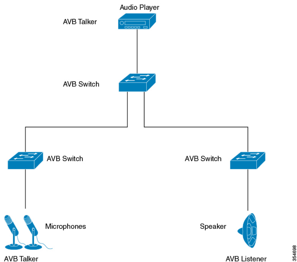
Figure 1: AVB network
